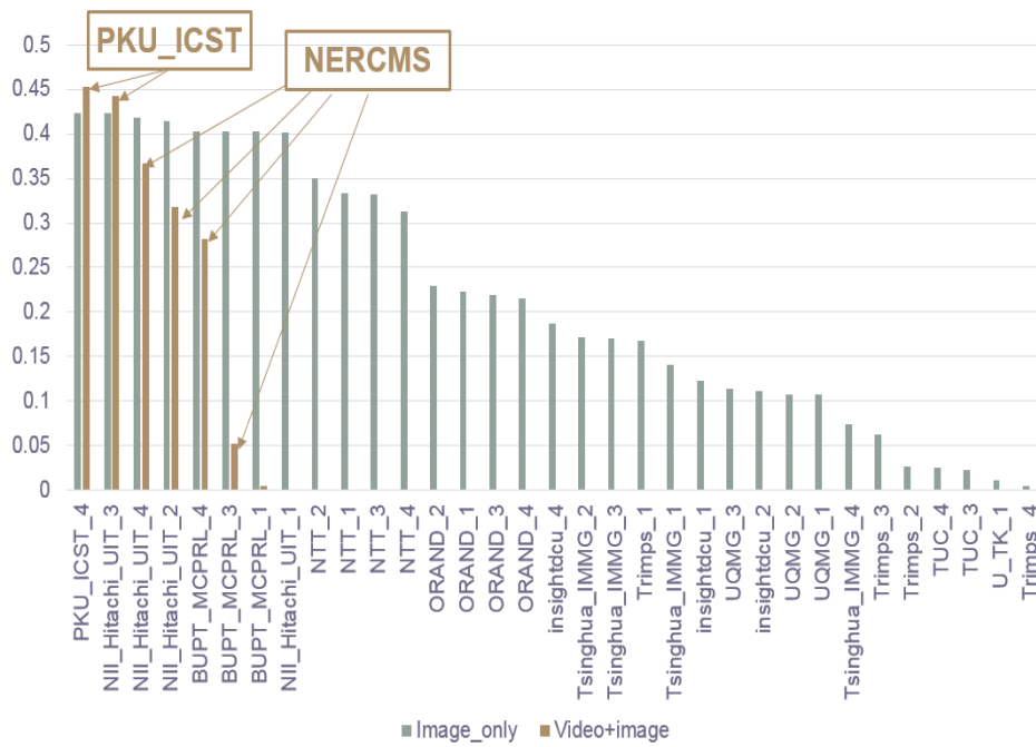
Figure 25: INS: Effect of number of topic example images used
