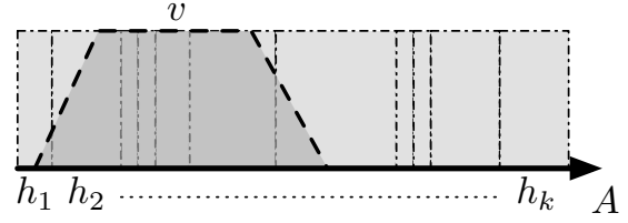
Fig. 2. Cardinality estimation of a term using a histogram about data distribution
