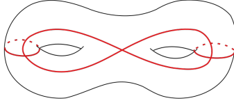
FIGURE 10 – One-faced collection with three curves
