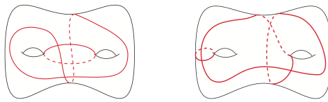
FIGURE 11 – One-faced collections with two curves
