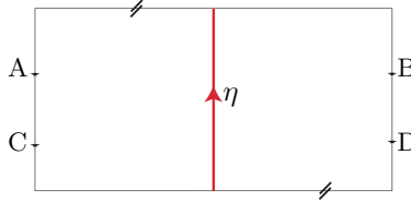
FIGURE 8 – End-points in annulus.
