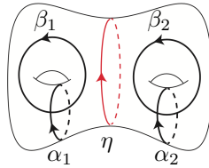
FIGURE 4 – Canonical symplectic basis.
