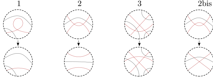
FIGURE 1 – From left to right, we have the three Reidemeister's moves and the last one is the crossing move (2bis) on which a bigon is replaced by a transverse self-intersection. The crossing move changes the homotopy class of the collection. The curves in red color represents the local configuration of \Gamma , and curves in black are sub-arcs of curves in \Sigma_g . One can see that Reidemeister's move 1 and 3 and crossing move do not change the intersection. Otherwise, the bigon deleting does change the intersection.
