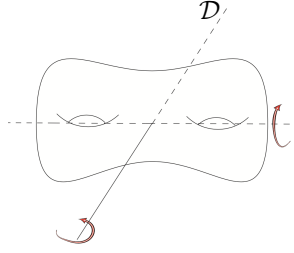
FIGURE 9 – Rotations R_1 and R_2
