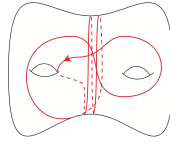
FIGURE 7 – The curve a_1\eta^2b_1^{-1}b_2
