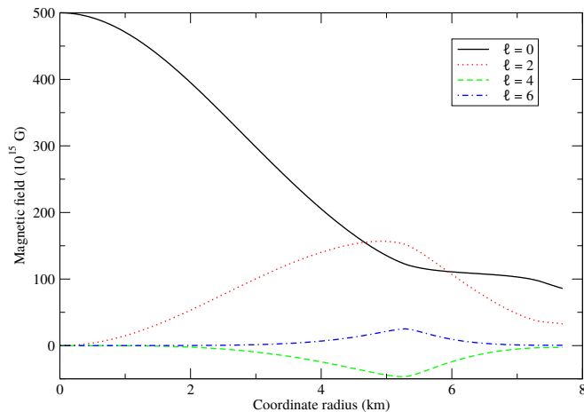
FIG. 3. Radial profiles of the first four even multipoles ( \ell = 0, 2, 4 and \ell = 6 ) of the magnetic field norm b(r, \theta) computed for the stellar model described in Fig. 1. From symmetry argument odd multipoles are all zero.
