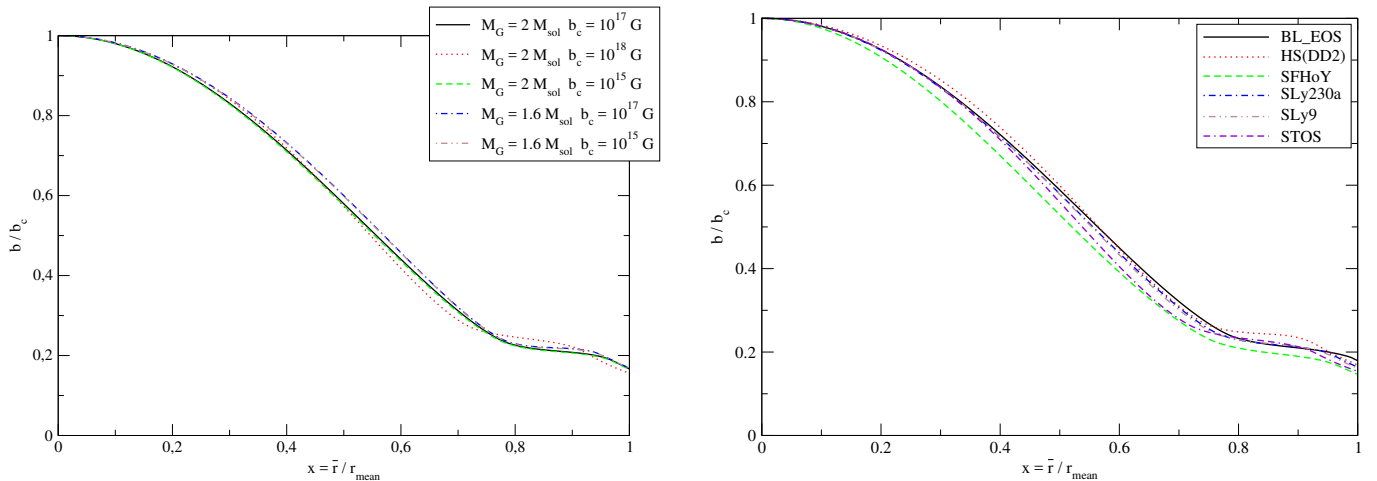
FIG. 4. Monopolar part of the magnetic field profile b_0(r) , normalized to its central value for different magnetized neutron star models, as functions of the radius expressed in Schwarzschild coordinates \bar{r} (see expression (5)) divided by the star’s mean radius (see text). Left panel: all models are using SLy230a EoS (see Tab. I) but have different masses ( 1.6 M_\odot or 2 M_\odot ) and different central magnetic fields ( 10^{15} G, 10^{17} G or 10^{18} G). Right panel: all are 2 M_\odot models, with a central magnetic field b_c = 5 \times 10^{17} G, but with different EoSs, see Tab. I for details.
