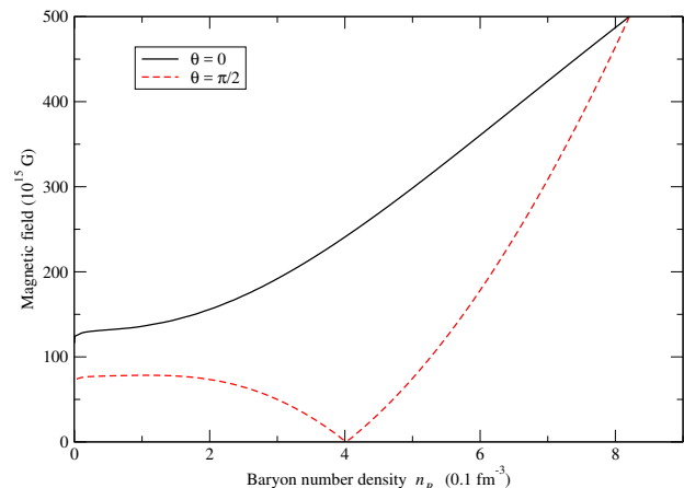
FIG. 2. Magnetic field norm as a function of the baryon density for two angular directions for the same stellar model as in Fig. 1.
