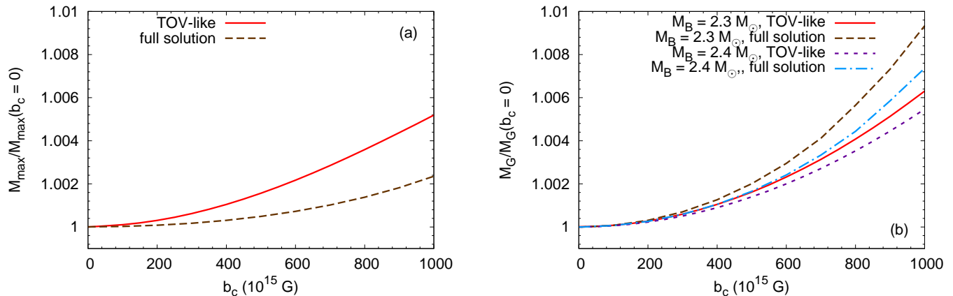
FIG. 6. (color online) Left: Comparing the values of the maximum gravitational mass as function of the central magnetic field between the TOV-like approach and the full solution. Right: Gravitational mass as function of the central magnetic field for two different values of the baryonic mass.
