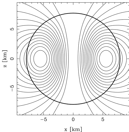
FIG. 1. Magnetic field lines in the (x, z) -plane for a M_G = 2 M_\odot neutron star model endowed with a magnetic field which central value is b_c = 5 \times 10^{17} G and using the SLy230a EoS of Tab. I. Thick line denotes the surface of the star and the magnetic moment is along the z -axis.
