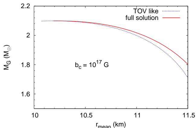
FIG. 5. (color online) Gravitational mass vs. mean radius for the TOV-like solution and the exact calculation for a central magnetic field of b_c = 10^{17} G and the SLy230a EoS.
