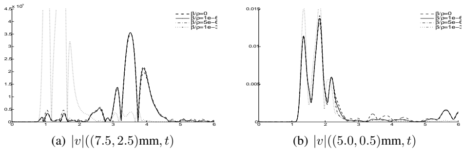
Figure 9: The modulus of the velocity |v|(\mathbf{x}_1, t) , t \in [0, 6] \mu s computed using the Q_1^{div} \times P_1^{disc} element with h = 0.025 \text{ mm} and different values of the damping parameter \beta .
