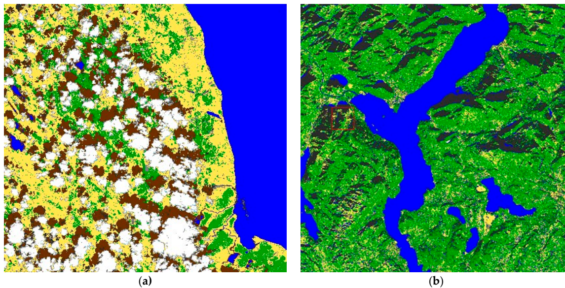
Figure 61. (a) Cloud shadows classification; (b) Topographic shadows classification.
