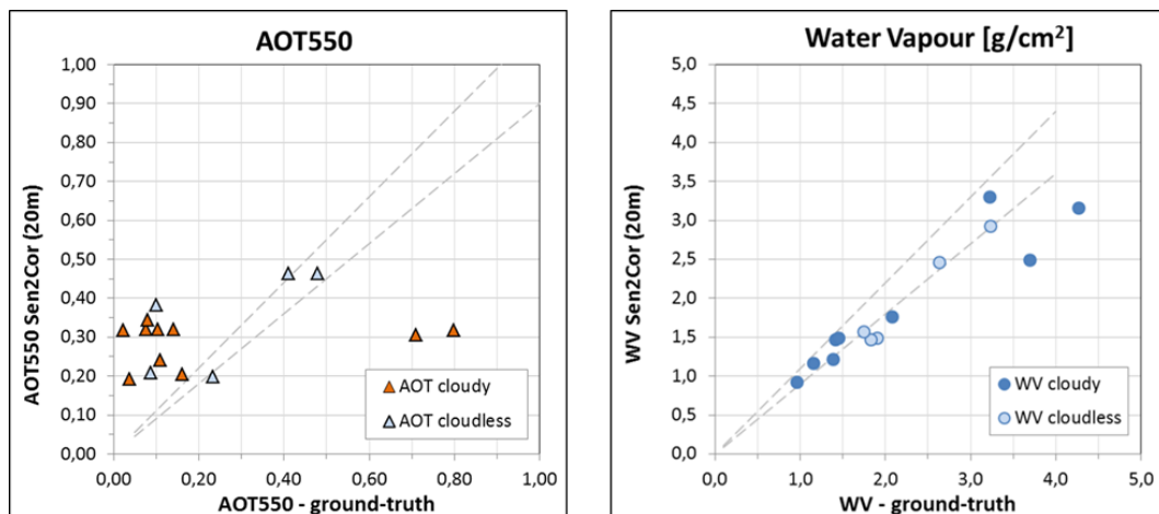
Figure 63. AOT and Water Vapour (WV) Validation. Direct comparison of Sen2Cor with ground reference from AERONET. Sen2Cor is represented by average over 9 \text{ km} \times 9 \text{ km} area with AERONET sunphotometer in the centre. Filled symbols represent samples with cloudiness >5\% and not filled with cloudiness <5\% .
