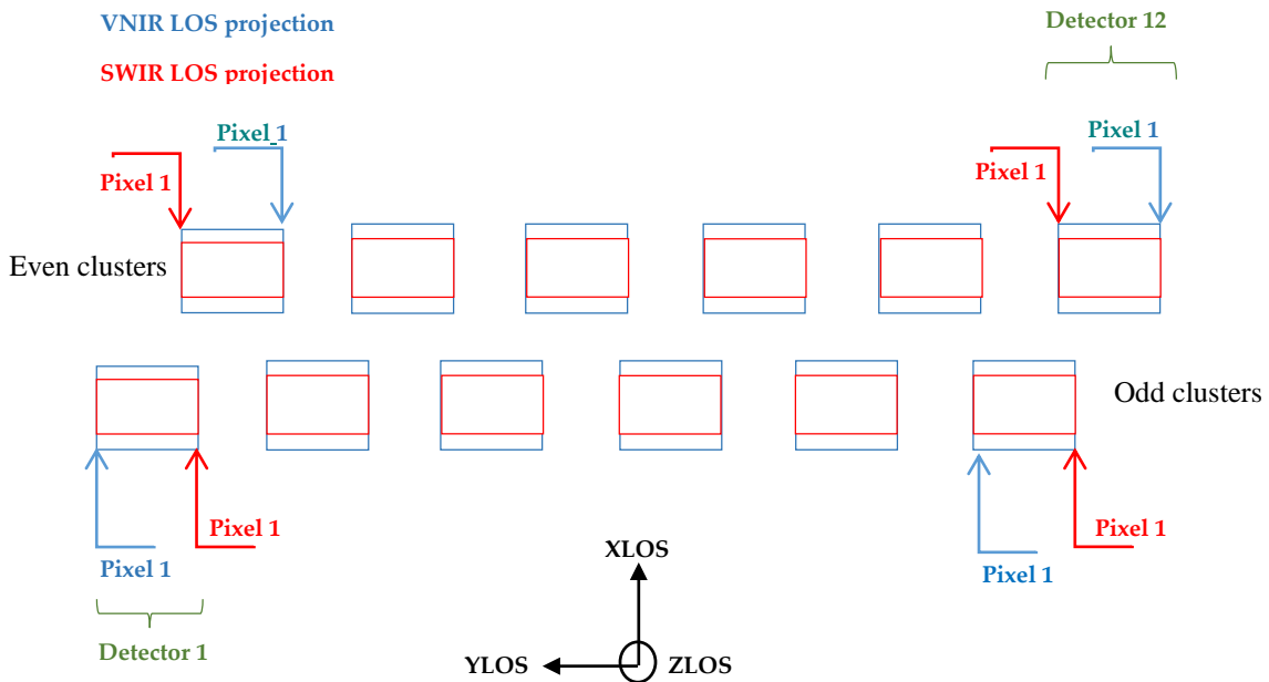
Figure 5. Representation of the pixels Line-Of-Sight (LOS) projection on ground.
