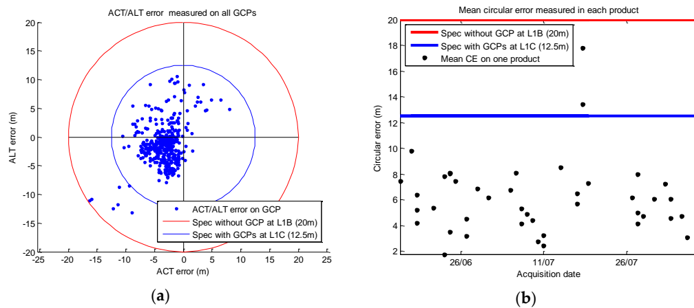
Figure 46. System Geolocation Performances in metres for L1C non-refined products. Reference band is B04. (a) Geolocation error (in metre) along-track and across-track measured on each GCP; (b) Mean geolocation error in each product processed in function of the acquisition dates of the product. The two outliers seen on both figures correspond to products from orbit 5601 and are due to contingencies (star-tracker outage).
