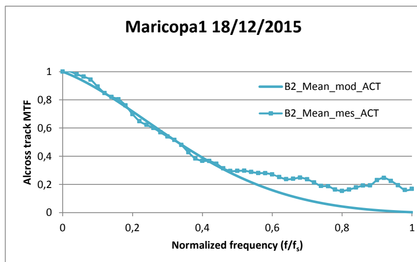
Figure 40. Modulation Transfer Function (MTF) curve for B02 band (centred at 490 nm) for the across-track direction.
