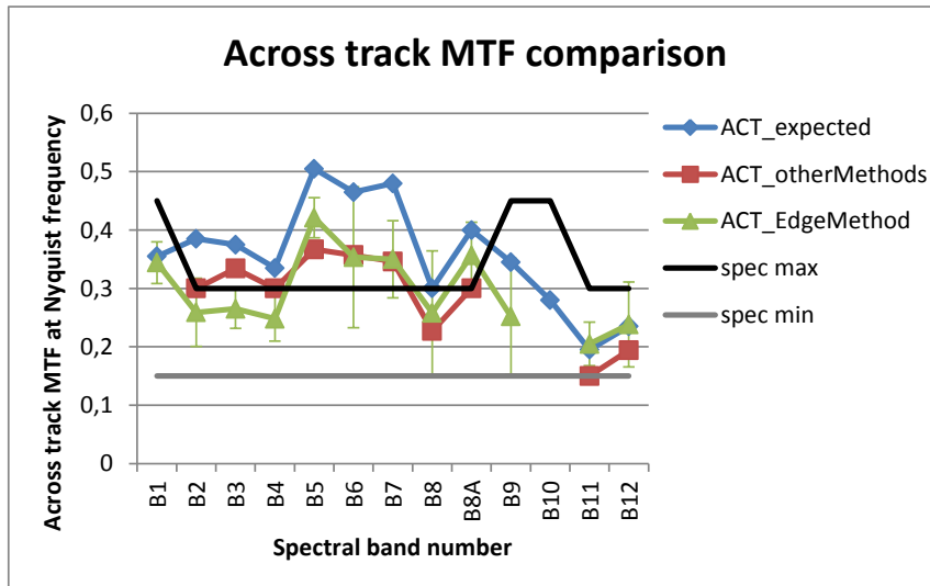
Figure 41. MTF results for the across-track direction, and MTF requirements (min value, spec min and max value, spec max).
