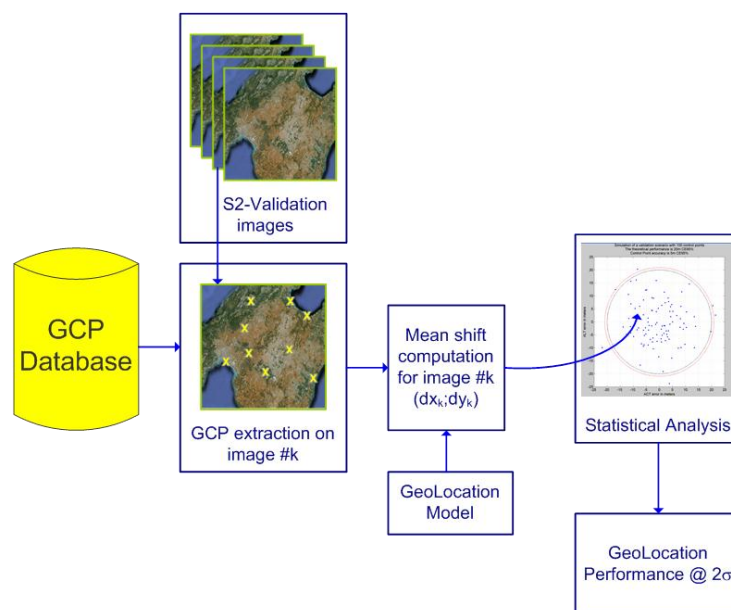
Figure 43. General principle of geolocation uncertainty validation using ground control points. Mean shift computation is obtained by correlation technique.
