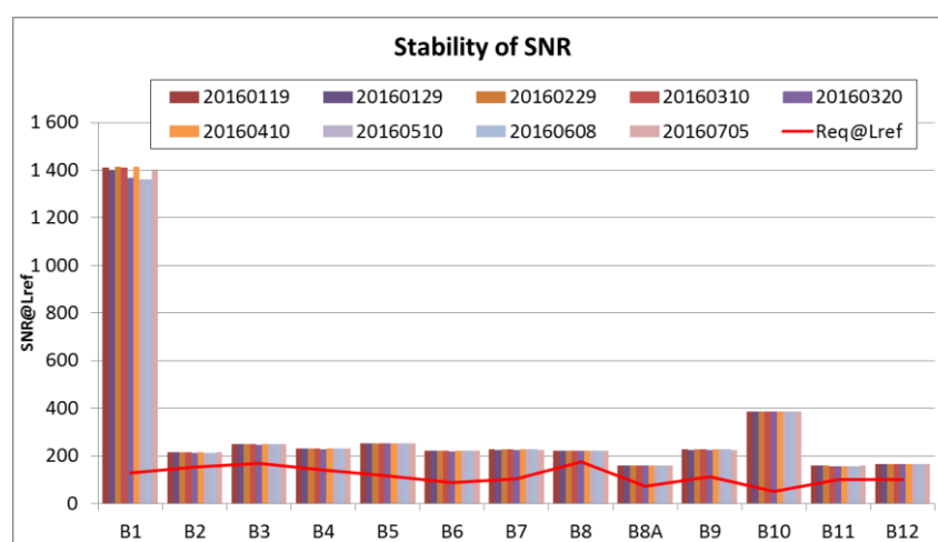
Figure 39. Average SNR at reference radiance L_{ref} measurements (per band) since January 2016.
