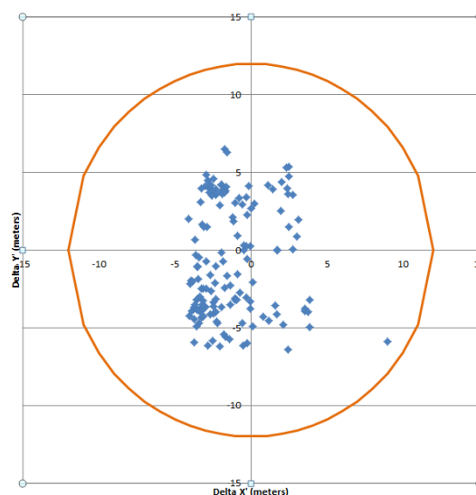
Figure 47. Product Geolocation Performances in metres (Band 04) for L1C refined tiles. Orange circle is the requirement with geometric refinement on GCPs.
