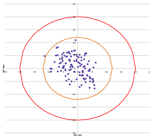
Figure 45. System Geolocation Performances in metres (Band 04) for L1B non-refined products. Red (resp. orange) circle is the requirement without (res. with) geometric refinement on GCPs.
