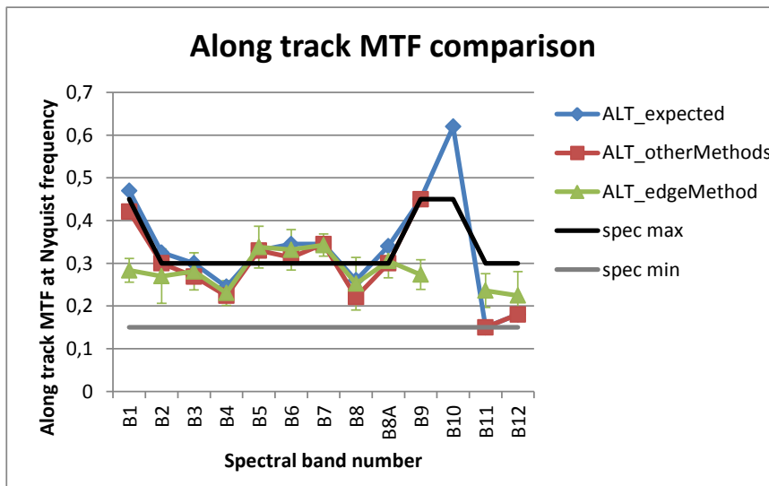
Figure 42. MTF results for the along-track direction, and MTF requirements (min value, spec min and max value, spec max).
