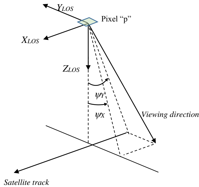
Figure 4. Line of Sight angles definition.
