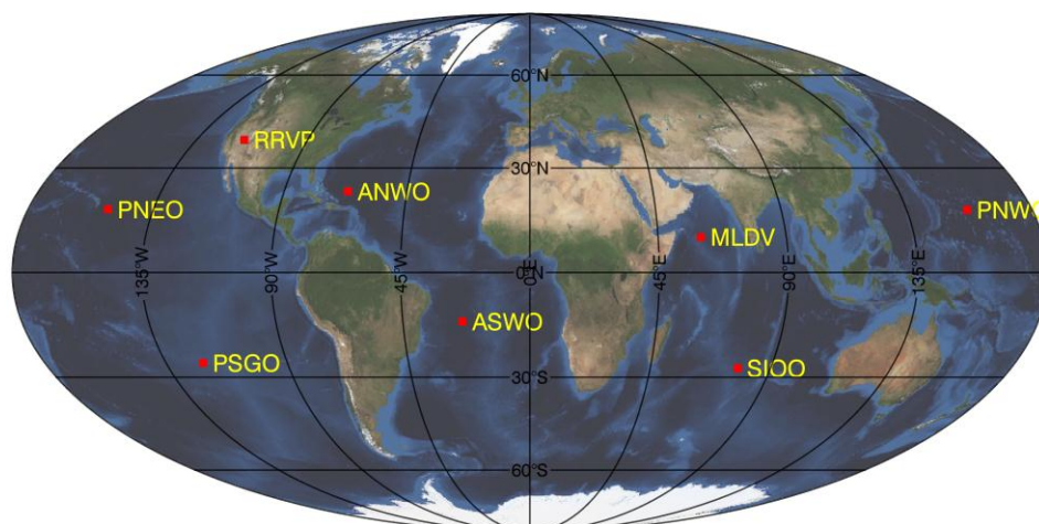
Figure 27. Cal/Val test sites location for Rayleigh scattering, Deep Convective Clouds (DCC), and ground-based methods chosen for Sentinel-2A commissioning activities. ANWO: Atlantic NW-Optimum, ASWO: Atlantic SW-Optimum, PNEO: Pacific NE-Optimum, PNWO: Pacific NW-Optimum, PSGO: Pacific Southern-Gyre-Optimum, SIOO: South-Indian Ocean-Optimum, MLDV: Maldives and RRVP: Rail-Road Valley Playa. (world image is taken from http://visibleearth.nasa.gov ).
