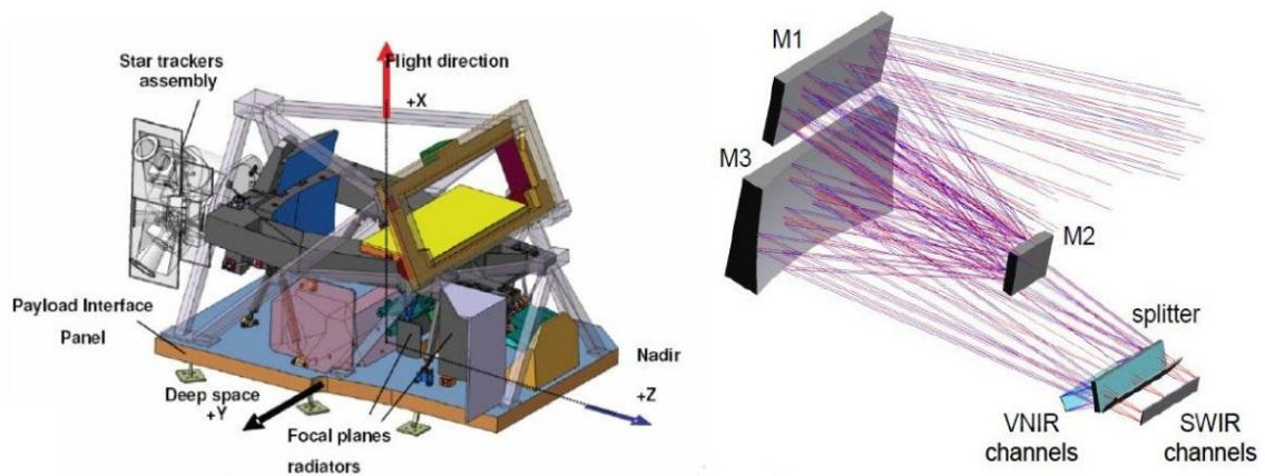
Figure 1. Multi-Spectral Instrument (MSI) internal configuration. Left: full instrument view (diffuser panel in yellow, telescope mirrors in dark blue). Right: optical path construction to the Short-Wave Infrared (SWIR)/visible to near-infrared (VNIR) (see Section 2.2) splitter and focal planes.
