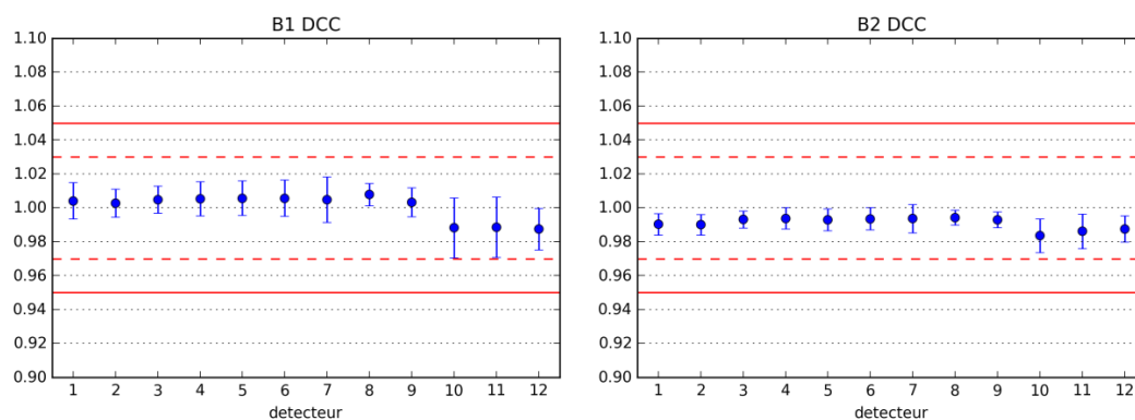
Figure 30. B01 (left) and B02 (right) inter-band calibration coefficients with respect to B04 as a reference band as a function of the detector number, based on Sentinel-2 images calibrated using the diffuser.
