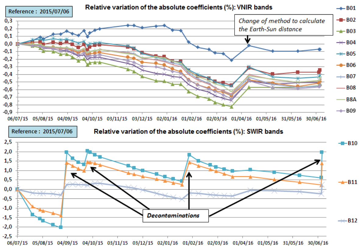
Figure 12. Time variation of the absolute calibration coefficients (for the processing baseline version 02.04), normalized to the coefficients estimated from the first Sun-diffuser acquisition performed on 06 July 2015.
