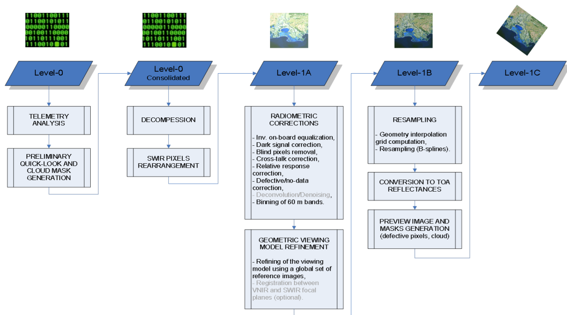
Figure 8. MSI processing chain overview. The gray font indicate optional steps implemented to mitigate risk on instrument performance but currently not activated.
