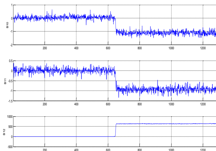
Figure 14. Characterisation of the electrical crosstalk: example of test result from ground measurement at Focal Plane Assembly (FPA) level (digital counts vs. pixel number).
