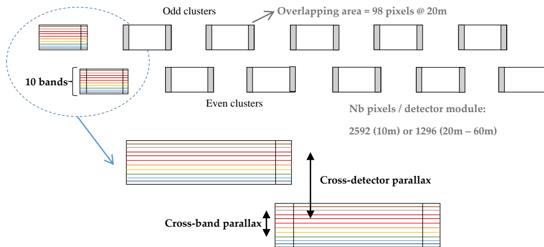
Figure 3. Staggered Detector Configuration.
