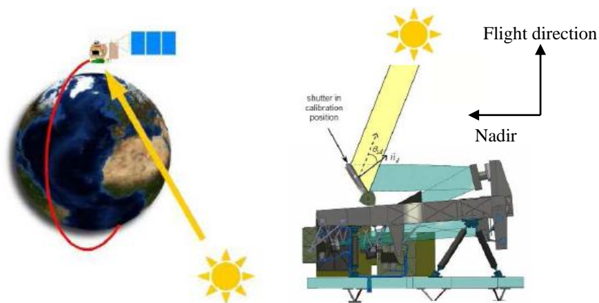
Figure 7. Illustration of the sun diffuser acquisition principle.
