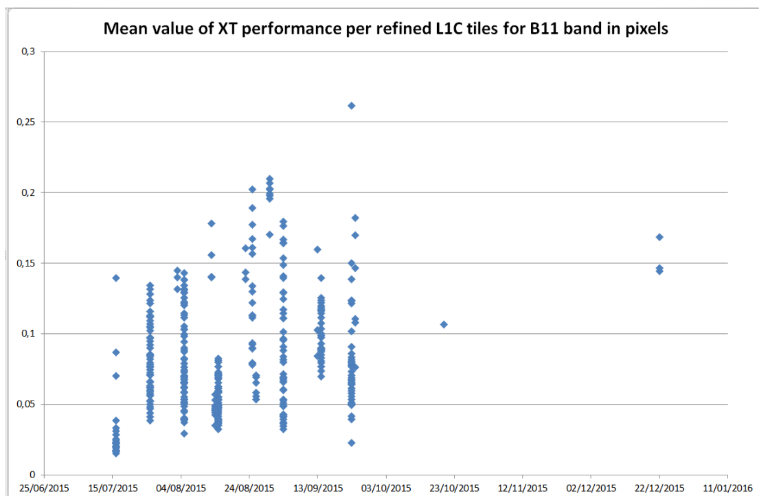
Figure 55. Multi-temporal (XT) registration uncertainty for B11 band. Each point represents the average shift measured in one secondary tile with respect to the reference tile.
