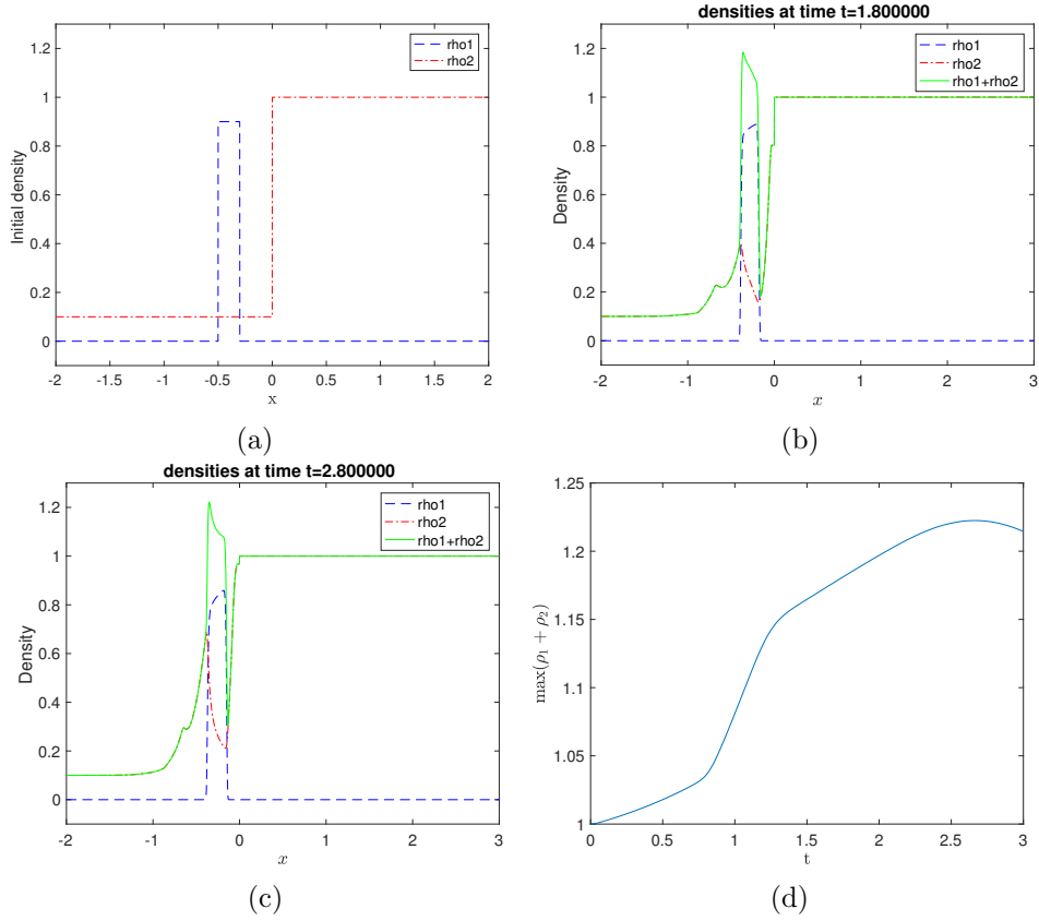
Figure 1: Numerical simulation illustrating that the simplex \mathcal{S} is not an invariant domain for (1.1). We take M = 2 and we consider the initial conditions \rho_1(0, x) = 0.9\chi_{[-0.5, -0.3]} and \rho_2(0, x) = 0.1\chi_{]-\infty, 0]} + \chi_{]0, +\infty[} depicted in (a), the constant kernels \omega_1(x) = \omega_2(x) = 1/\eta , \eta = 0.5 , and the speed functions given by v_1^{max} = 0.2 , v_2^{max} = 1 , \psi(\xi) = \max\{1 - \xi, 0\} for \xi \geq 0 . The space and time discretization steps are \Delta x = 0.001 and \Delta t = 0.4\Delta x . Plots (b) and (c) show the density profiles of \rho_1 , \rho_2 and their sum r at times t = 1.8 , 2.8 . The function \max_{x \in \mathbb{R}} r(t, x) is plotted in (d), showing that r can take values greater than 1, even if r(0, x) = \rho_1(0, x) + \rho_2(0, x) \leq 1 .
