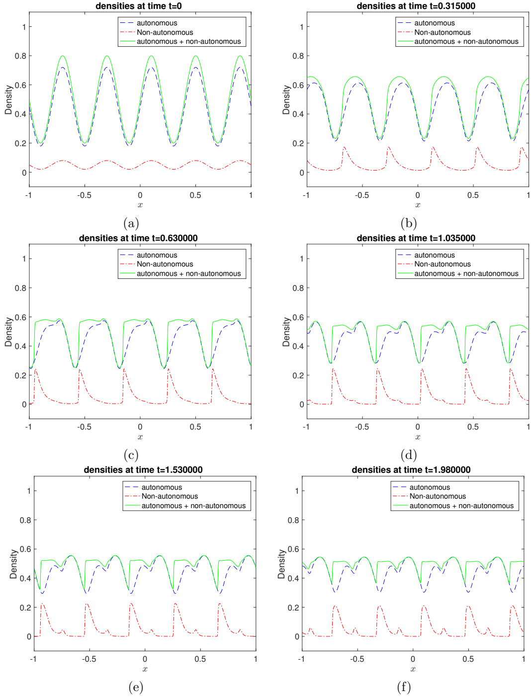
Figure 3: Density profiles corresponding to the non-local problem (4.2) with \beta = 0.9 at different times.
