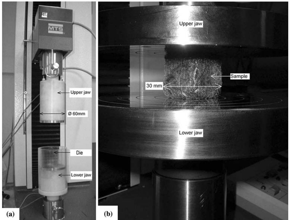
Fig. 5 a Specific device for compression on entangled fibers, and b device for cross-linked fibers
