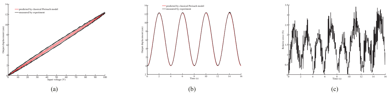
Fig. 12. Hysteresis responses with sinusoid voltages of amplitude 100 V (a) hysteresis loops (b) time responses (c) relative error between the measured and predicted curves
