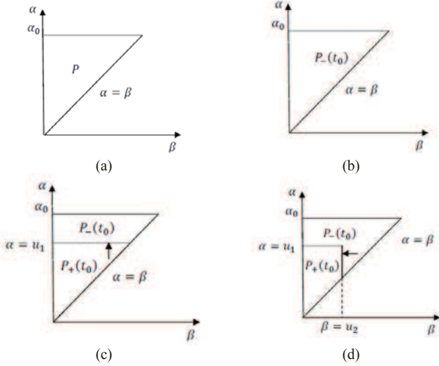
Fig. 3. Memory curve in the Preisach plane
