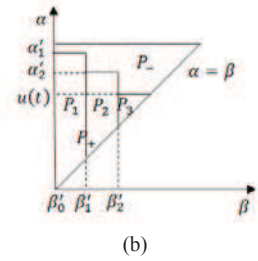
Fig. 6. (a) Hysteresis loop with several extrema \alpha'_k and \beta'_k (b) the region P_k corresponding to (a)
