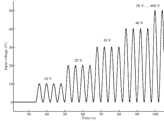
Fig. 10. A sine piecewise voltage signal used to identify classical Preisach model
