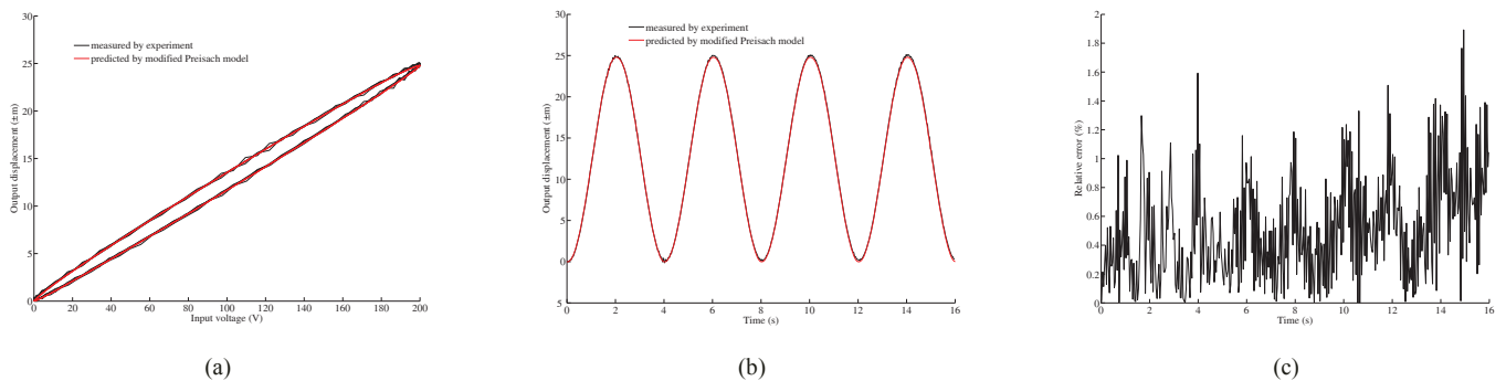
Fig. 15. Hysteresis responses with sinusoid voltages of amplitude 200 V (a) hysteresis loops (b) time responses (c) relative error between the measured and predicted curves
