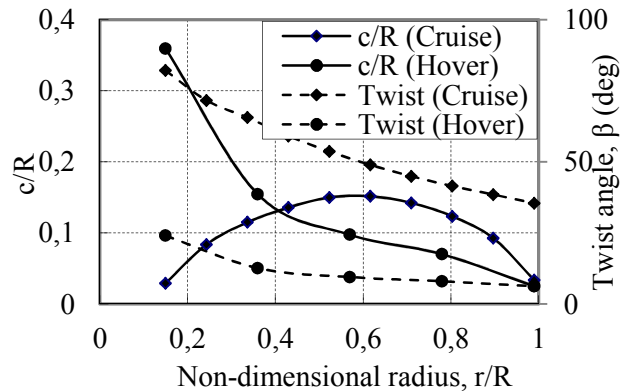
Fig. 11 Optimal blade shapes at single design point in hover and in cruise
