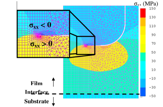
Fig. 20. Stress field ( \sigma_{xx} ) around the crack tip at 80^\circ\text{C} ( r = 5 \mu\text{m} , W = 10 \mu\text{m} , a = 9 \mu\text{m} , E_{\text{film}} = 32 \text{ GPa} ).
