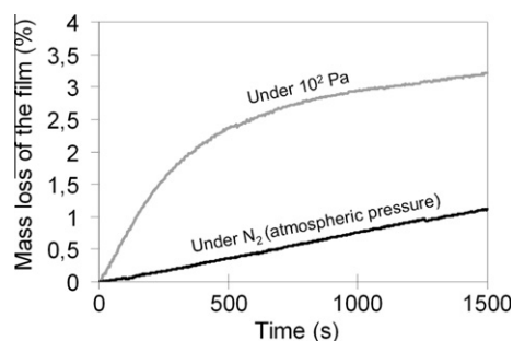
Fig. 5. Thermo-gravimetric analysis of anodic films with initial porosity of 40% at ambient temperature.
