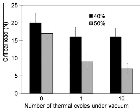
Fig. 8. Evolution of the scratch-test critical load as a function of the number of thermal cycles between -80 and +80 °C under vacuum ( 10^{-6} Pa).
