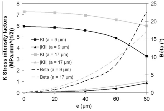
Fig. 18. Stress intensity factors and bifurcation angle of the central crack as a function of its eccentricity ( a = 9 \mu\text{m} or a = 17 \mu\text{m} , T = 120^\circ\text{C} and E_{\text{film}} = 32 \text{ GPa} ).
