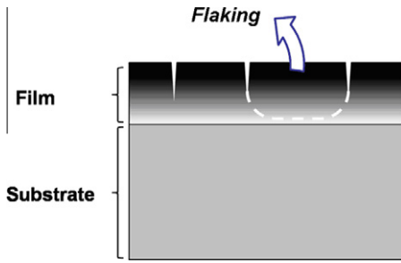
Fig. 13. Schema of crack propagation in an anodic film leading to flaking.
