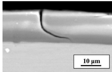
Fig. 19. Schema of the numerical model with a kinked crack (on the left) and comparison with SEM cross-section view (on the right).
