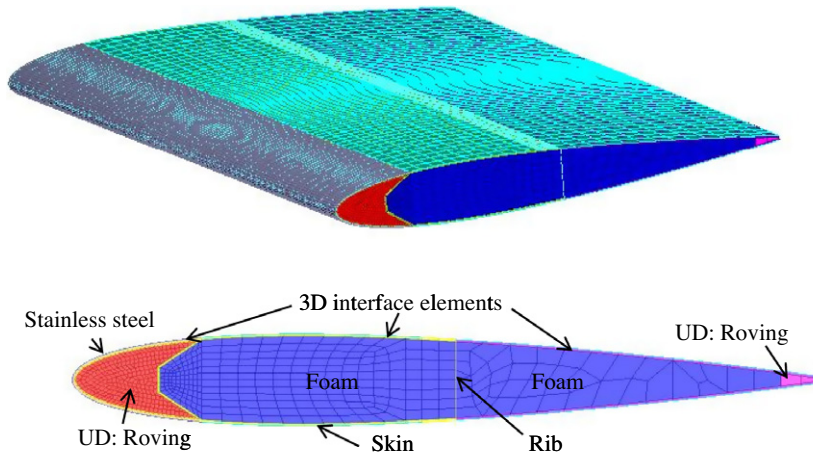
Fig. 8. Specimen mesh.
