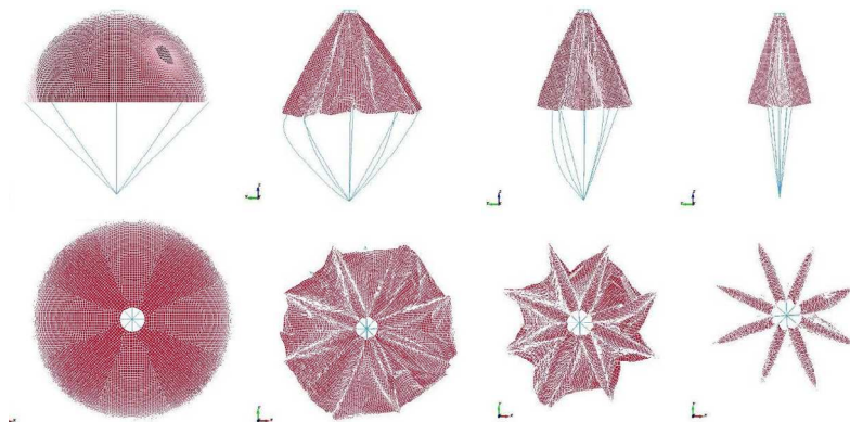
Figure 10. Parachute forming process using added mass.
