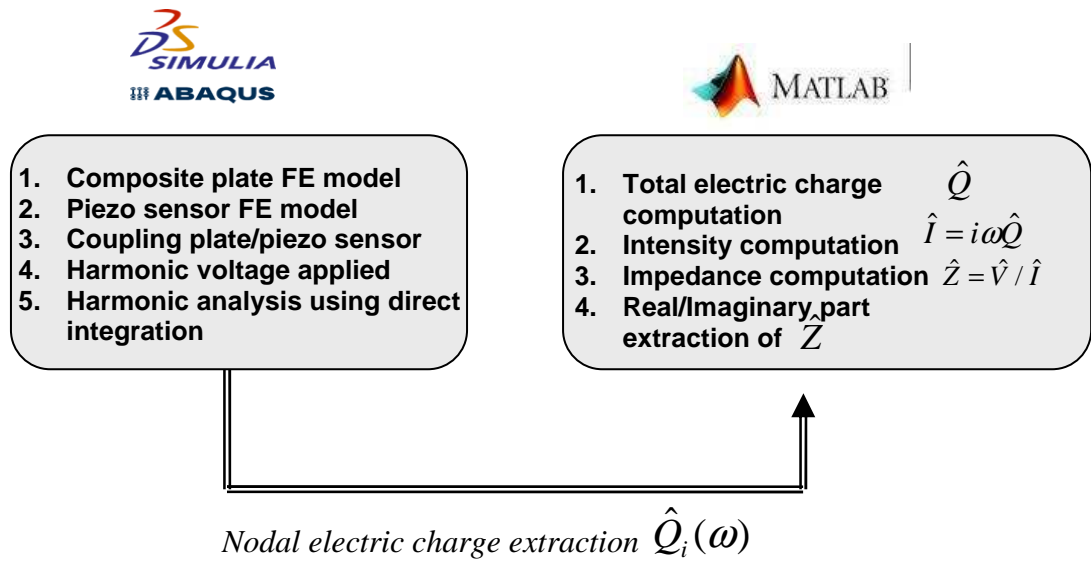
Figure 1: Modeling principle of the EMI technique.
