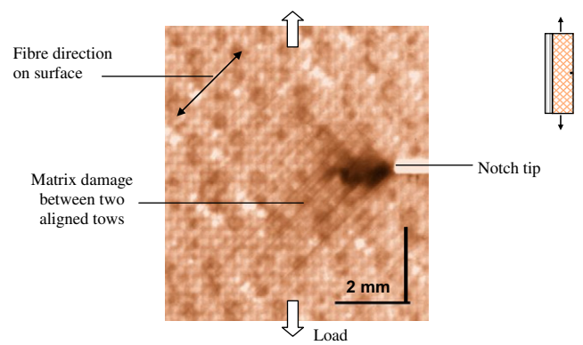
Fig. 8. Crack length after 5 \times 10^6 cycles in [45]_2 notched laminate loaded in fatigue.
