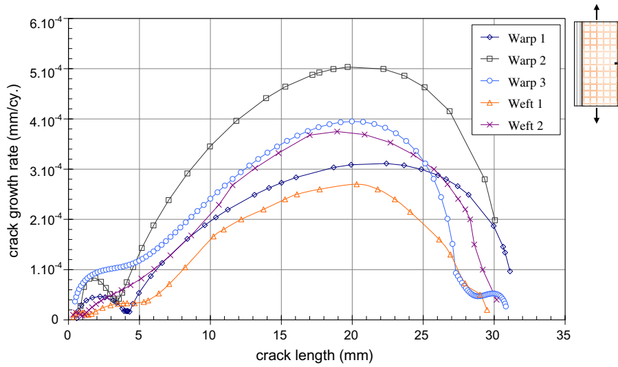
Fig. 6. Crack growth rates versus crack length in warp [0]_2 and weft [90]_2 laminates in samples of 50 mm width.
