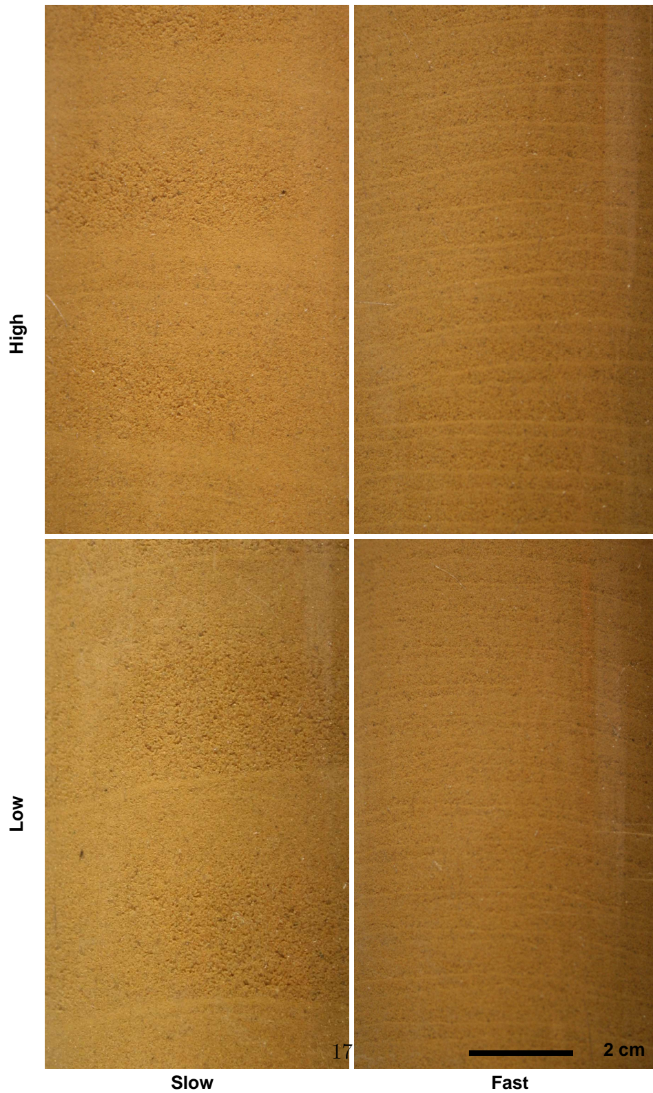
Figure 5: Pictures of SSC-1 prepared in transparent container with Rain method. The layering and segregation of particles in each layer are visible in each picture. The differences in soil fabric caused by the slow or fast speed of the hopper are clearly visible. A fast hopper speed creates thin layers and a slow hopper speeds creates thick layers. Hopper height has no visible influence on layering.
