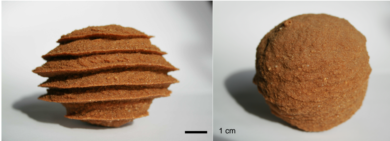
Figure 8: Pictures of resin spheres obtained after preparing and impregnating SSC-1. The spheres have a diameter of approximately 5 cm. On the right, the round resin sphere is a poured SSC-1 sample. On the left the resin “sphere” is a rained sample (Scott (2009)). The resin impregnation technique allows local fabric observation.
