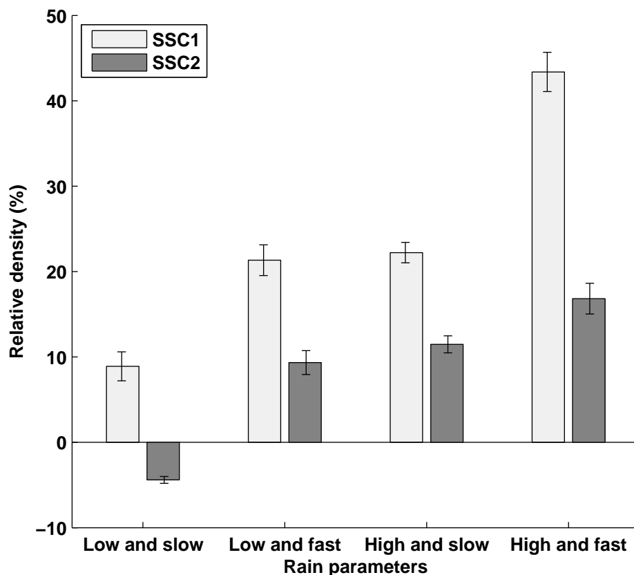
Figure 4: Mean value of volumetric relative density data set measured after using Rain preparation techniques on SSC-1 and SSC-2 to fill a 245 mL cylindrical container. The speed of hopper and height of hopper were varied.
