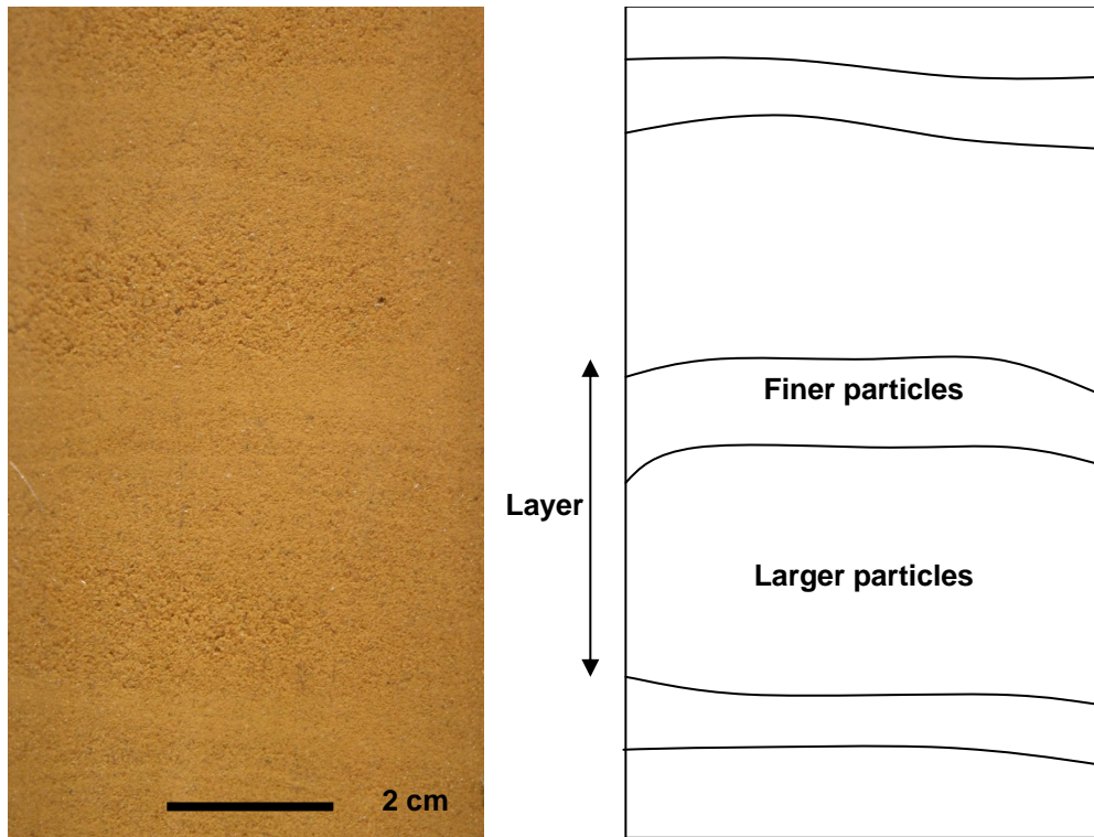
Figure 6: Picture and schematic of SSC-1 prepared in transparent container with Rain method from high height at low hopper speed. The schematic highlights the position of the different layers and the segregation in each layer.
