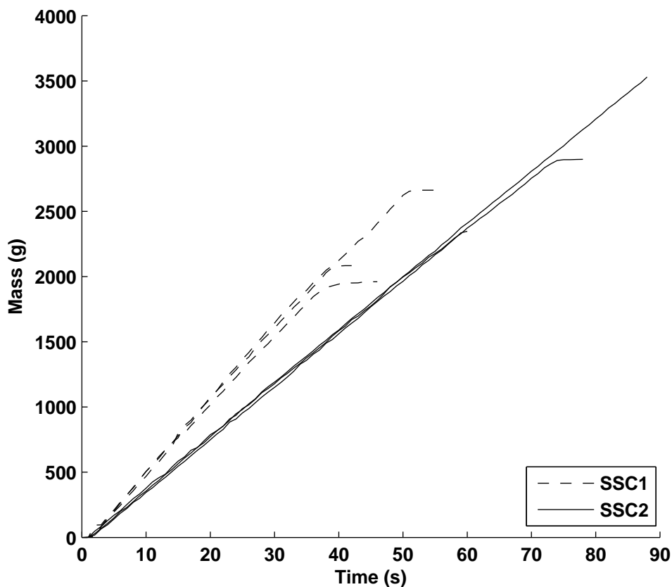
Figure 2: Graph of cumulative mass obtained when raining SSC-1 and SSC-2 regolith simulants from the hopper.
