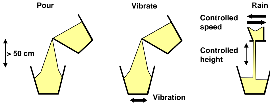
Figure 1: The three Granular Material (GM) preparation techniques explored in this publication: Pour (from a height above 50 cm), Vibrate (while pouring the GM in container) and Rain (a curtain of GM is deposited by layers from a controlled height and at a controlled speed).
