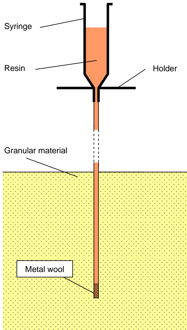
Figure 3: Schematic of resin impregnation set-up with needle placed in the granular material and filled with resin.
