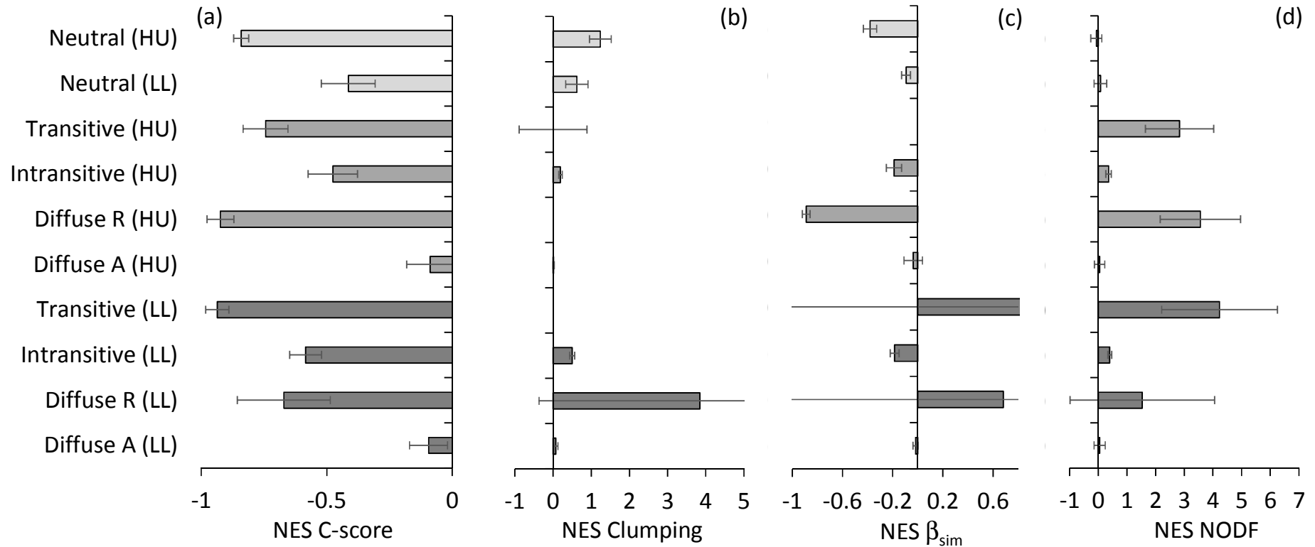
37 Figure 4. Normalized effects sizes NES (equiprobable null model) the C-core (a), the clumping score (b), \beta_{sim} (c), and NODF (d) for neutral 38 models with high migration probability and unlimited dispersal (HU, grey bars) and low migration probability and limited dispersal (LL, dark 39 grey) for neutral communities (light grey) for those with additional transitive and intransitive competition hierarchies, and diffuse competition 40 penalizing rare (Diffuse R) and abundant (Diffuse A) species. Error bars are one standard deviation obtained from 10 replicates each. 41
