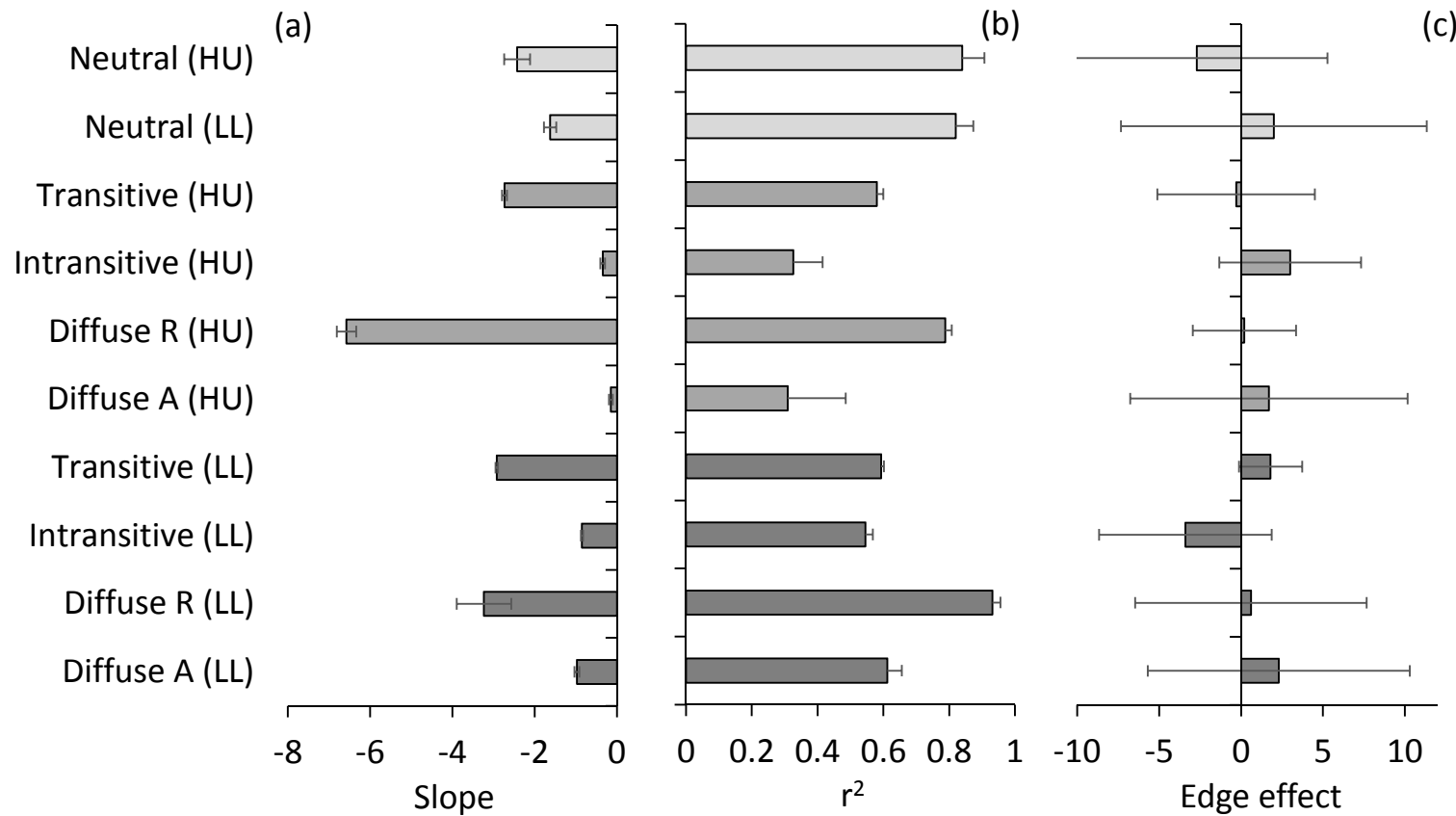
23 Figure 2. Average slope of the exponential species decay curve (a), and the respective coefficient of determination r^2 (b), and the effect of grid 24 edges (c) for neutral models with high migration probability and unlimited dispersal (HU, grey) and low migration probability and limited 25 dispersal (LL, dark grey) for neutral communities (light grey) and for neutral communities with additional transitive and intransitive competition 26 hierarchies, and diffuse competition penalizing rare (Diffuse R) and abundant (Diffuse A) species. Error bars are one standard deviation. 27
