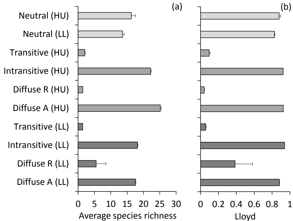
29 Figure 3. Average species richness (a), and the spatial variability in richness as quantified by the index of Lloyd (b) for neutral models with high 30 migration probability and unlimited dispersal (HU, grey) and low migration probability and limited dispersal (LL, dark grey) for neutral 31 communities (light grey) and for neutral communities with additional transitive and intransitive competition hierarchies, and diffuse competition 32 penalizing rare (Diffuse R) and abundant (Diffuse A) species. Error bars are one standard deviation. 33
