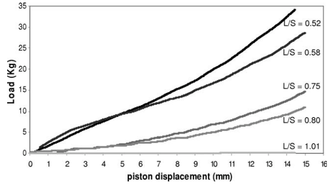
FIGURE 7. Influence of the L/S ratio on the load (in kg) to apply on the piston to extrude the reference paste at room temperature.
