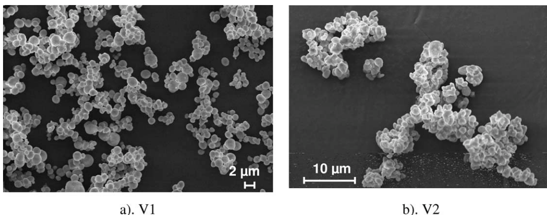
FIGURE 3. SEM micrographs of the two types of vaterite synthesized.
