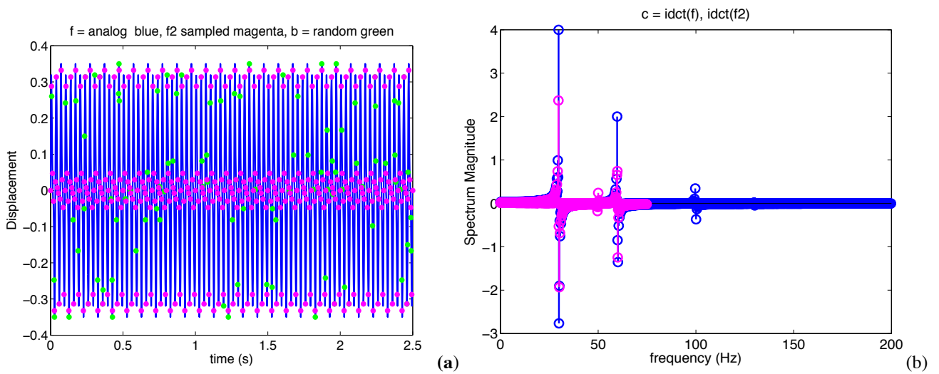
Fig. 2. Analog signal (in blue), discretized signal (magenta) respecting Nyquist frequency (N points) and randomized signals at low resolution (N/10) (a), and DCT spectrum comparison (b)
