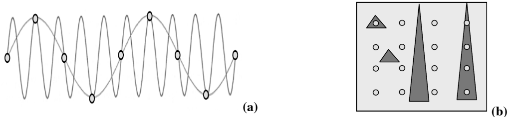
Fig. 5.: In general artefacts are due to under-sampling or poor reconstruction: Temporal aliasing (Shannon's theorem) (a), Spatial aliasing (b) due to limited spatial resolution and induce loss of details.
