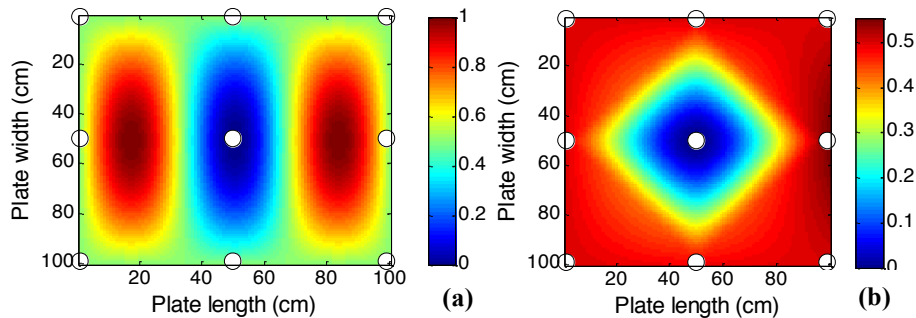
Fig. 1. : (3,1) mode of vibrating plate plus regular grid distribution of sensors in white circles (a) and The cubic interpolation which shows a spatial aliasing in mode shape reconstruction (b). A regular grid of 9 sensors permits only to reconstruct the (1,1).
