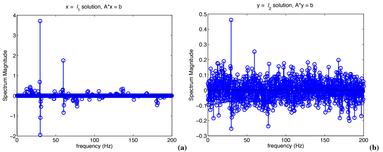
Fig. 3. Comparison of DCT spectrum of reconstructed signals by \ell_1 inversion (a) and \ell_2 inversion (b) of randomized signals. The \ell_2 inversion is not capable of good reconstruction (noise)
