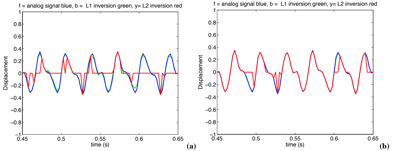
Fig. 4. Comparison of reconstructed signals by \ell_1 inversion (green) for different sampling N/10 (a) and N/5 : (b) of randomized signals. From the time domain (zoom) The \ell_2 inversion (red) is not capable of good reconstruction of the continuous signal (blue) whereas \ell_1 optimization (green) is reliable even for low sampling.
