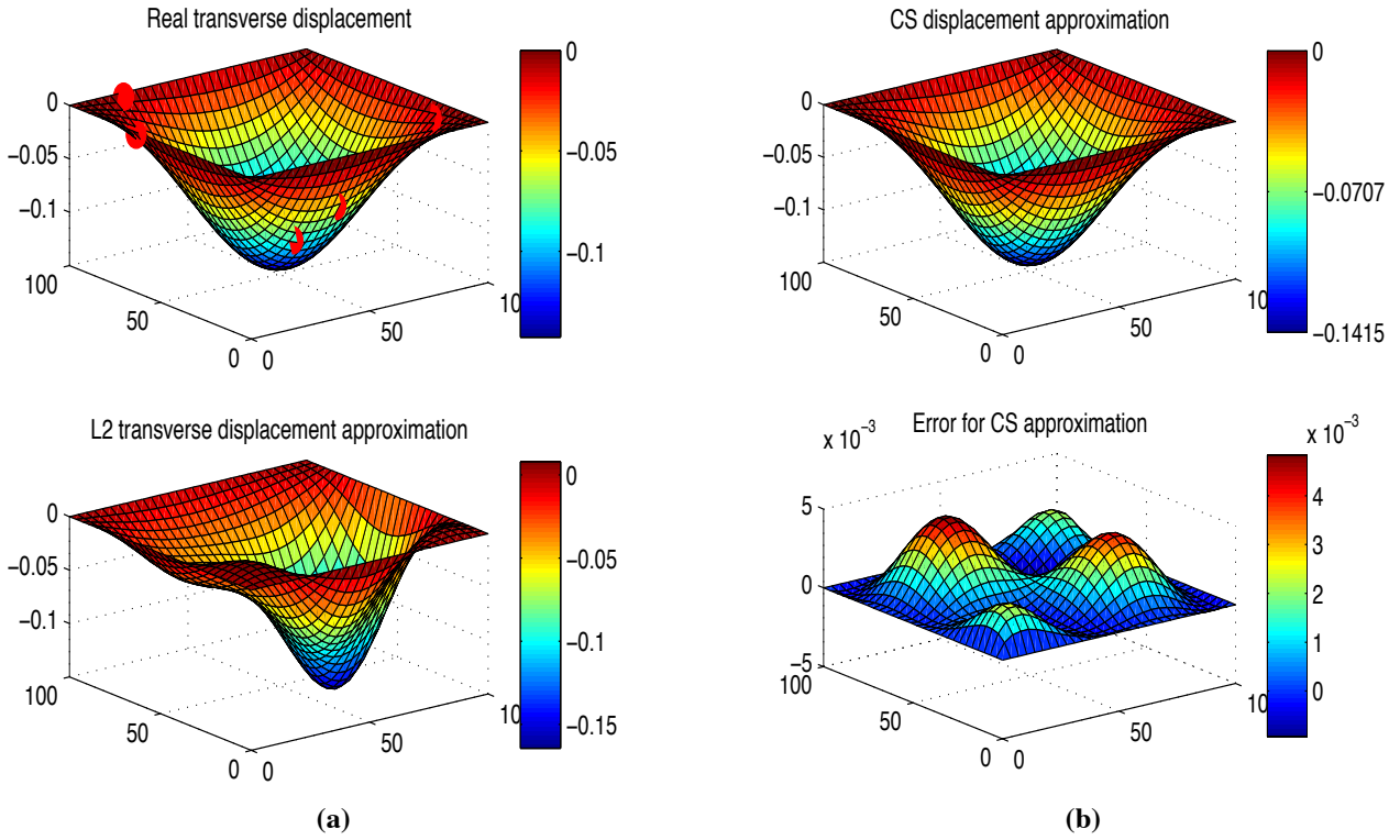
Fig. 6. First modeshape reconstruction of a SSSS plate. The sensors are in red (randomly chosen) on the ‘continuous’ modeshape (a) one can see the \ell_2 inversion results on bottom. (b) We demonstrate the CS ability to reconstruct the modeshape, on bottom one can see the error versus continuous modeshape (maximum error of 5E-3 ).
