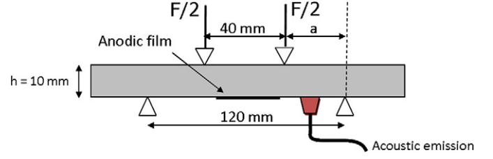
Fig. 1. Diagram of the four-point bending test monitored by acoustic emission.
