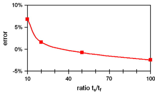
Fig. 3. Evolution of the error between Eq. (4) and results obtained by the numerical model as a function of the thickness ratio ( E_f = 50 GPa, T = 80 °C and \alpha_f = 5.10^{-6} \text{ K}^{-1} ).
