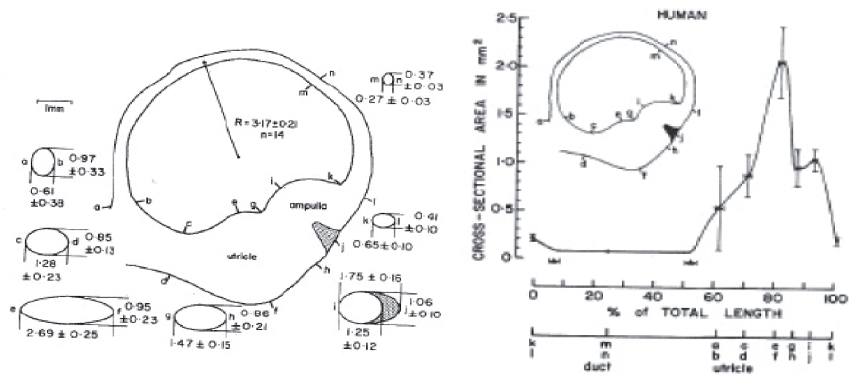
Figure 5: Horizontal Canal Geometry (Curthoys and Oman, 1987)
