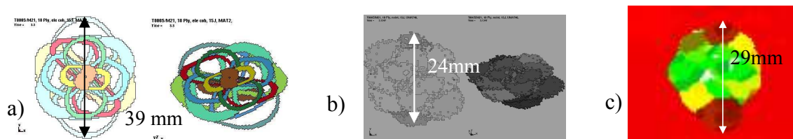
Figure 3. a) Delaminated cohesive or b) saturated elements model, and c) DT 15J C-Scan.
