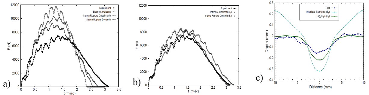
Figures 2. a) and b) Force [N] versus time [ms] history curves; c) Indentations [mm].
