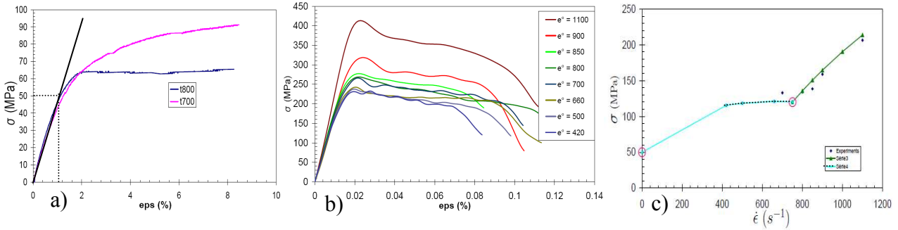
Figure 1. a) Quasi-static tension of T700/M21S and T800/M21S [\pm 45^\circ]_{2s} ; b) Dynamic compression of T800/M21S [\pm 45^\circ]_{3s} ; c) Strain rate effects on T800/M21S [\pm 45^\circ]_{2s} lamina strength.
