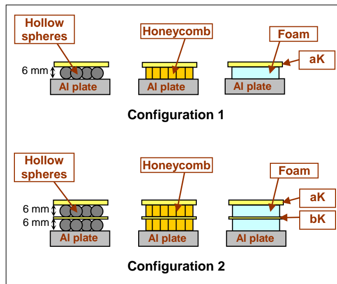
Figure 2 : Geometry and material configuration of protective layers
