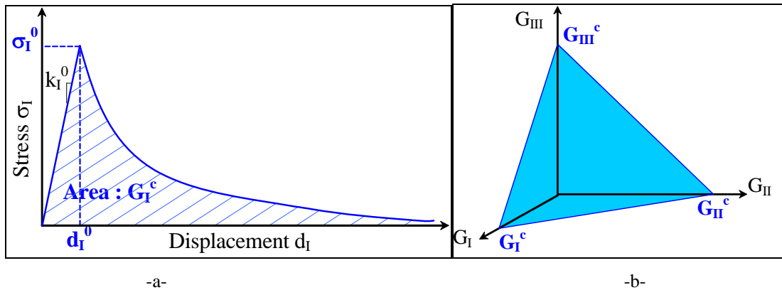
Figure 3. Softening law of the stress-displacement curve (a) and linear mixed mode of fracture (b)
