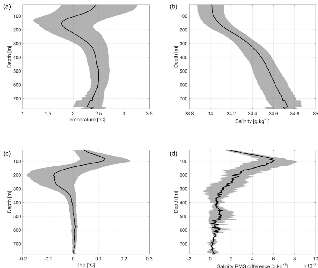
FIG. 7. (a) Mean temperature, (b) salinity, (c) T_{HP} , (d) RMS_{ad\_raw} - RMS_{ad\_cor} profiles averaged for all full-resolution CTD-SRD L tags deployed on SES around the Kerguelen Islands. The shaded area envelopes represent the 20th and 80th percentiles in all four plots.
