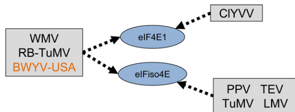
Figure 9 Update on the selective recruitment of translation initiation factors 4E by ssRNA+ viruses in Arabidopsis . Arrows indicate that the virus isolate relies on the 4E factor to infect the plant. WMV, Watermelon mosaic virus ; RB-TuMV, resistance-breaking Turnip mosaic virus ; CIYVV, Clover yellow vein virus ; PPV, Plum pox virus ; TEV, Tobacco etch virus ; LMV, Lettuce mosaic virus ; BWYV-USA, Beet western yellows virus-USA . Potyviruses are coloured in black and poleroviruses in orange.
