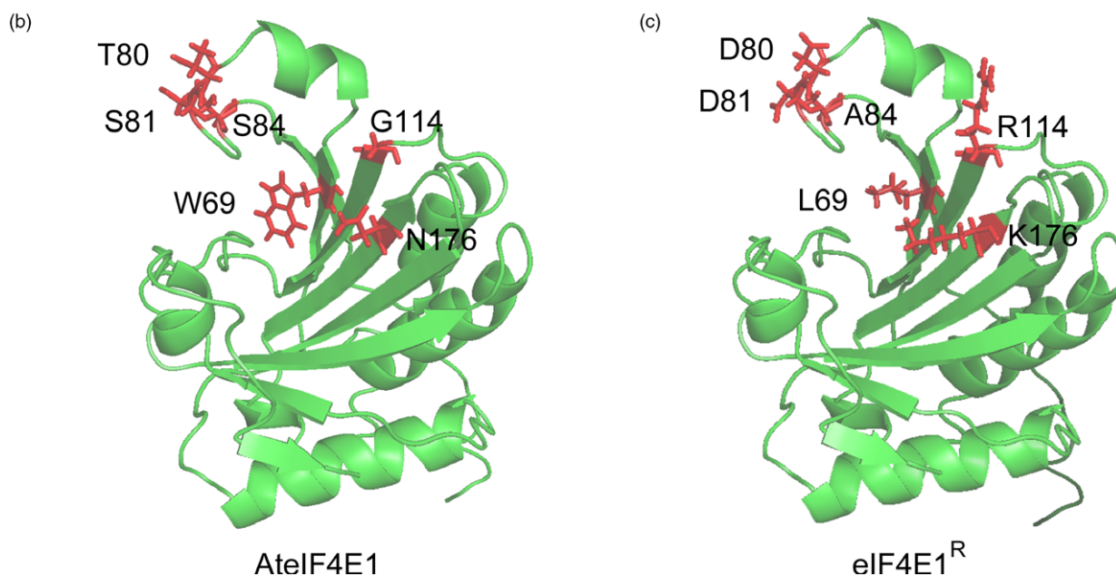
Figure 1 Design of a synthetic Arabidopsis resistance allele eIF4E1 R . (a) Alignment of eIF4E protein sequences from pea susceptible (JI2009) and resistant (JI1405 and PI269818) accessions with the Arabidopsis thaliana eIF4E1 (AteIF4E1). The position of the amino acids that differ between susceptible and resistance pea accessions is highlighted in grey. Black triangles above the alignment indicate the mutations introduced in Arabidopsis eIF4E1 to create the synthetic eIF4E1 R . (b and c) Three-dimensional predicted structure of AteIF4E1 (b) and of eIF4E1 R (c) based on homology modelling using the pea eIF4E 3D structure as a template (PDB ID: 2WMC-C). The modified amino acids between AteIF4E1 and eIF4E1 R are coloured in red with side chains shown.
