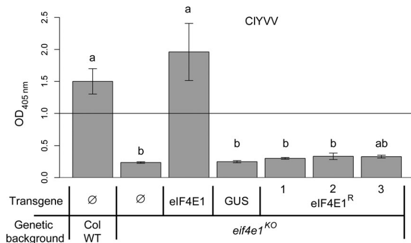
Figure 3 eIF4E1 R is a resistance allele to CIYVV in Arabidopsis . CIYVV accumulation in eif4e1 KO plants transformed with the wild-type eIF4E1 genomic construct under its own promoter ( eIF4E1 ), the GUS gene under the control of the 35S promoter (GUS) or with the genomic eIF4E1 R construct under its endogenous promoter (three independent lines are shown, eIF4E1 R 1–3). Wild-type Columbia and eif4e1 KO plants are used as positive and negative controls, respectively. Accumulation of CIYVV was assessed by DAS-ELISA 30 days postinoculation. (a) and (b) represent significantly different groups, P < 0.05 .
