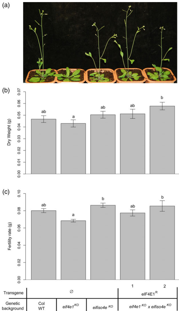
Figure 4 eIF4E1 R complements the eif4e1 KO eifiso4e KO lethality phenotype at no developmental cost. (a) Phenotype of two independent eif4e1 KO eifiso4e KO eIF4E1 R lines, four weeks after sowing. (b) Dry weight analyses of 4-week-old controls and eif4e1 KO eifiso4e KO eIF4E1 R plants. Results were averaged from 20 plants for each genotype. (c) Fertility rate is the weight of seeds produced by plants of controls lines and eif4e1 KO eifiso4e KO eIF4E1 R plants. Results were averaged from 10 plants for each genotype. Kruskal–Wallis statistical tests were performed to identify statistically significant differences (a) and (b) represent significantly different groups ( P < 0.05 , standard error bars are represented on the graph).
