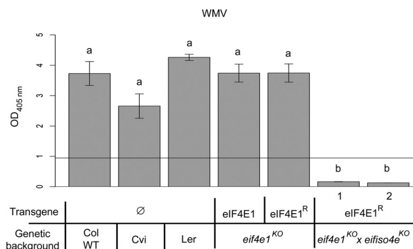
Figure 6 eif4e1 KO eifiso4e KO eIF4E1 R plants resistance spectrum extends to WMV. WMV viral accumulation was measured by DAS-ELISA in control lines and in two eif4e1 KO eifiso4e KO eIF4E1 R lines. DAS-ELISA was performed at 21 days after inoculation with WMV. a and b represent significantly different groups, P < 0.05 .
