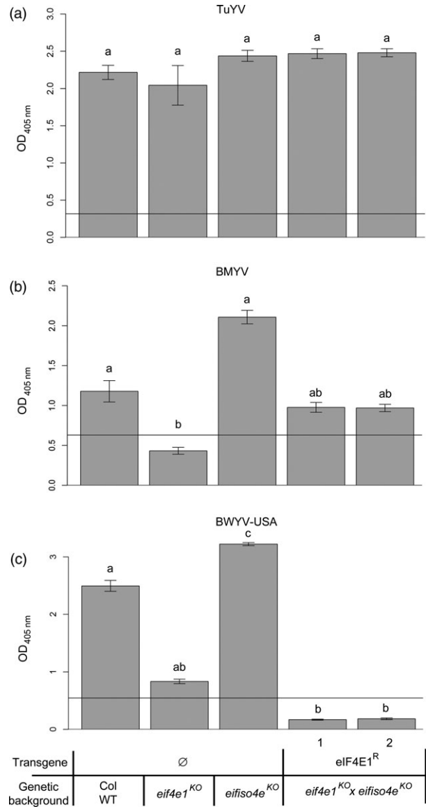
Figure 8 eif4e1 KO eifiso4e KO eIF4E1 R plants resistance spectrum extends to polerovirus species BWYV-USA but not to TuYV and BMVY. BWYV-USA, TuYV and BMVY viral accumulation was measured by DAS-ELISA in control lines and in two eif4e1 KO eifiso4e KO eIF4E1 R lines. DAS-ELISA was performed 21 days after inoculation with TuYV (a), BMVY (b) or BWYV-USA (c). 12 plants per genotype were tested, and experiments were repeated twice. a, b and c represent significantly different groups, P < 0.05.
