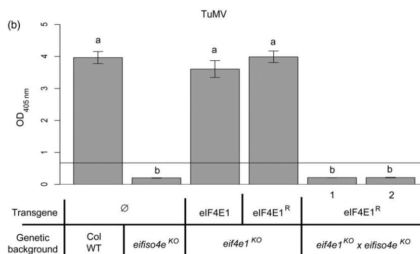
Figure 5 eif4e1 KO eifiso4e KO eIF4E1 R plants cumulate the respective resistances to TuMV and CIYVV. CIYVV and TuMV viral accumulation measured by DAS-ELISA in control lines and in two eif4e1 KO eifiso4e KO eIF4E1 R lines. DAS-ELISA was performed 30 days after inoculation with CIYVV (a) or 21 days after inoculation with TuMV (b). a, b and c represent significantly different groups, P < 0.05 .
