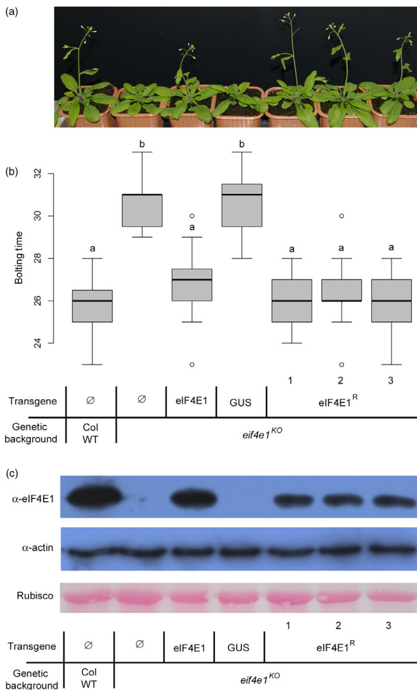
Figure 2 Functional complementation of eif4e1 KO plants by eIF4E1 R allele. (a) Bolting of eif4e1 KO and complemented plants, 4 weeks after sowing. Columbia Wild-type plants (Col WT) are used as control. Results are shown for three independent transgenic lines (1 to 3) expressing the eIF4E1 R construct in a eif4e1 KO background. Table legend shown under (b) applies also for (a). (b) Boxplot representation of the bolting time (in days after sowing) for the same genotypes as in (a). Results are averaged from 16 individual plants per genotype. (a) and (b) represent significantly different groups ( P < 0.05 ). (c) In planta cap-binding purification of eIF4E1 proteins. Total soluble protein extract from control and transgenic plants was purified on m7GTP-agarose beads. After purification, the output fraction was analysed by Western blot using anti-eIF4E1 antibody while equal loading control was checked on total protein (input) by Western blot for actin detection and by Ponceau staining for Rubisco protein detection.
