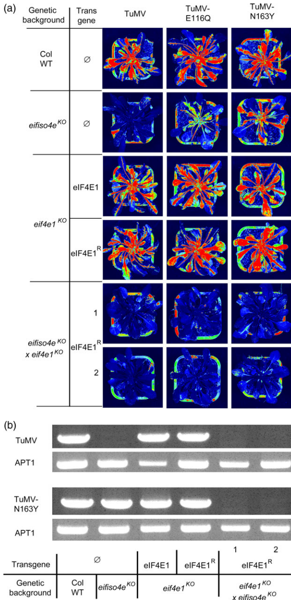
Figure 7 eif4e1 KO eifiso4e KO eIF4E1 R plant resistance spectrum extends to resistance-breaking TuMV isolates. Controls and eif4e1 KO eifiso4e KO eIF4E1 R lines were challenged with either GFP-tagged TuMV, GFP-TuMV-E116Q (RB) or GFP-TuMV-N163Y (RB). Viral accumulation was assessed using GFPcam (PSI) camera-imaging (a). Fluorescence intensity is shown in false colour from blue (low) to red (high intensity) with the plant pot reflecting light, allowing visualization of the outline of the plant position. (b) Detection of TuMV mRNA by RT-PCR amplification of the VPg coding sequence for both TuMV-GFP and TuMV-N163Y-GFP 21 dpi in the noninoculated leaves. ADENINE PHOSPHORIBOSYL TRANSFERASE 1 ( APT1 ) gene was used as a control for RNA extraction.
