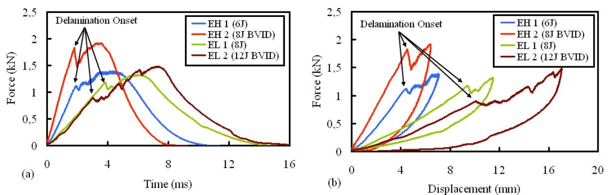
Fig. 5. Impact test data (a) force-time (b) force-displacement
