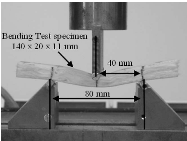
Fig. 3. Test specimen between the three supports during three-point bending test.
