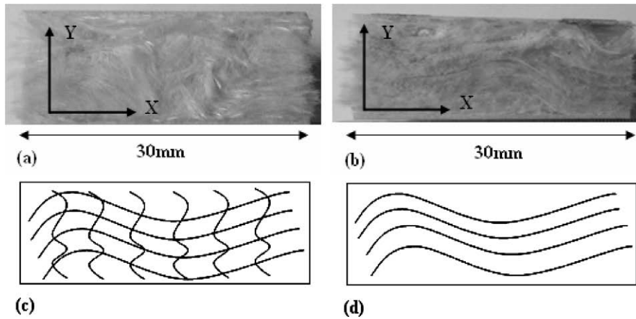
Fig. 8. Cross-section view of specimen showing the orientation of fibers: (a) 10 mm fiber length entangled sandwich specimen, (b) 15 mm fiber length entangled sandwich specimen. Schematic view explaining the orientation of fibers (c) 10 mm fiber length entangled sandwich specimen and (d) 15 mm fiber length entangled sandwich specimen.
