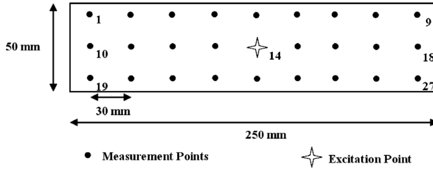
Fig. 6. Location of excitation and measurement points in sandwich beam for vibration test.
