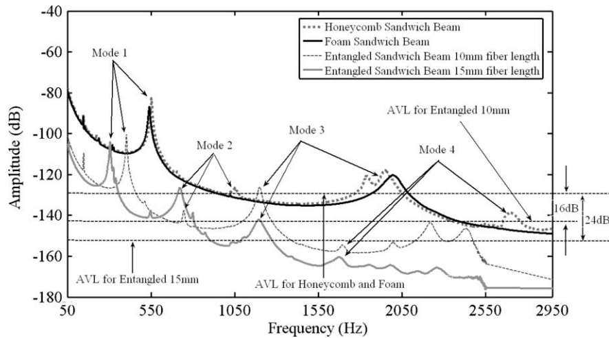
Fig. 10. Comparison of the Sum of frequency response function (FRF) for the honeycomb, foam and entangled sandwich specimens with the average vibratory level.
