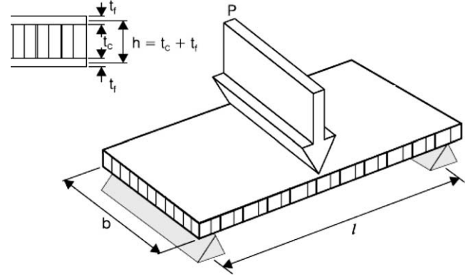
Fig. 4. Sketch of a sandwich beam under three-point bending showing geometrical parameters.
