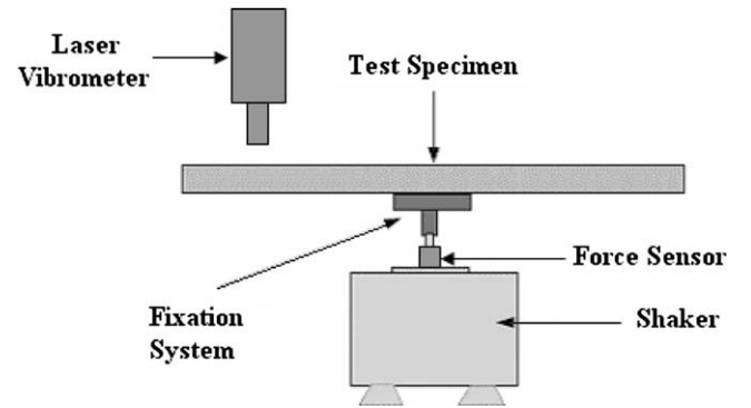
Fig. 5. Diagram of the experimental set-up for vibration testing.
