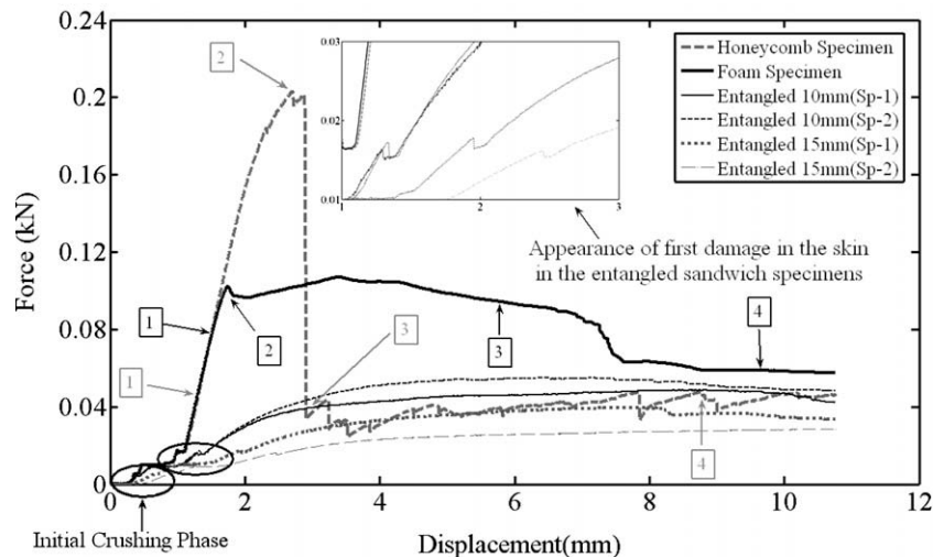
Fig. 9. Force–deflection curves measured under three–point bending tests for the entangled (10 and 15 mm fiber core length), foam and honeycomb sandwich specimens. The appearance of the first damage in the skins is indicated.
