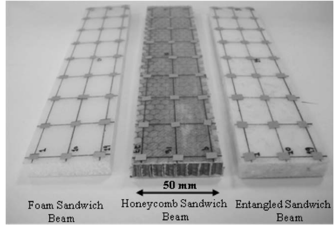
Fig. 1. Sandwich test specimens with honeycomb, foam and entangled glass fibers as core used for vibration testing.
