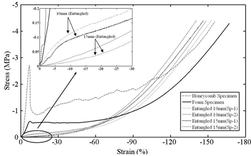
Fig. 7. Compression stress/strain curves for the entangled (10 and 15 mm fiber core length), foam and honeycomb sandwich specimens. The zoomed view shows the linear-elastic phase used for calculating the elastic modulus.
