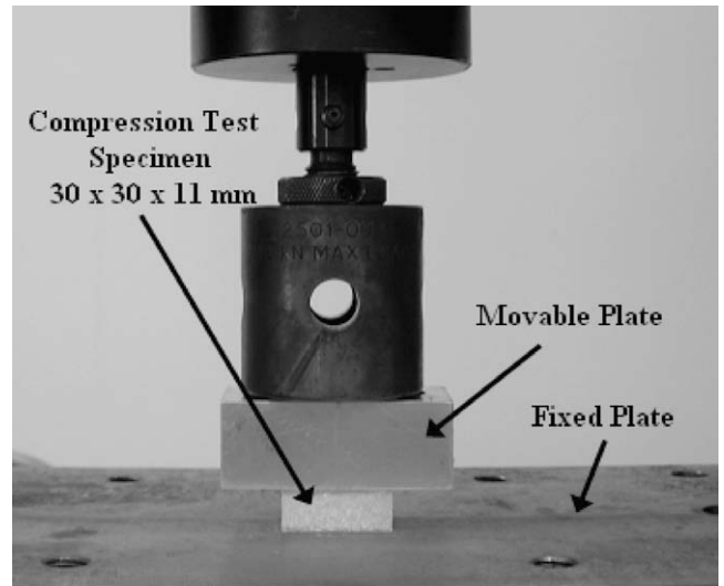
Fig. 2. Test Specimen between the fixed and moveable plate during compression test.
