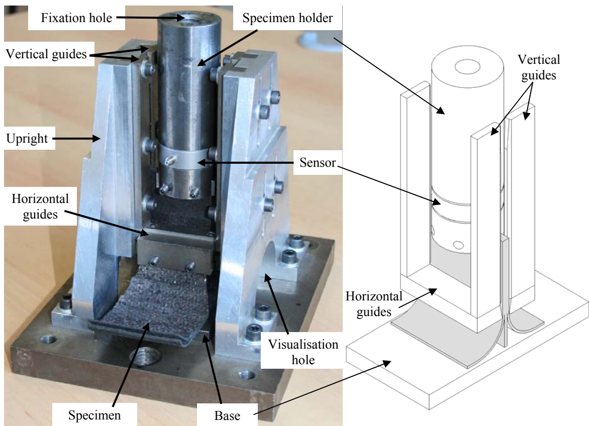
Figure 1: Test fixture: photo and simplified drawing (without uprights)
