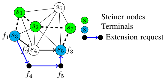
Fig. 1: A Steiner-based tree for E-SFC placement
