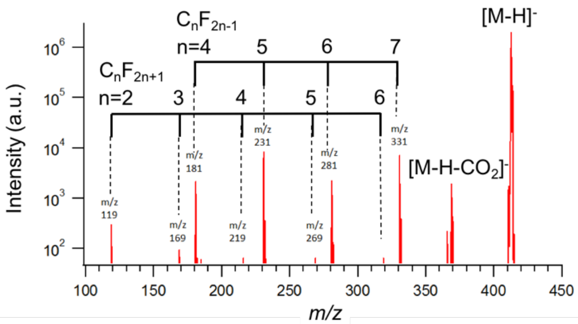
Figure 2. Mass spectrum of the selected [PFOA - H]^M- ion after activation at 8 eV (155 nm).
