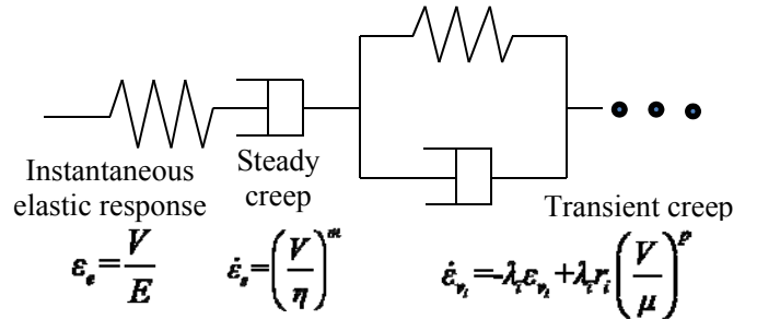
Fig. 4 The phenomenological model for creep
