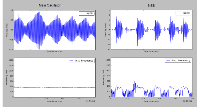
FIGURE 2: Deterministic excitation : Response on main oscillator (left) and NES (right)- Transient response (Top view) and Instantaneous Frequency (Bottom view)
