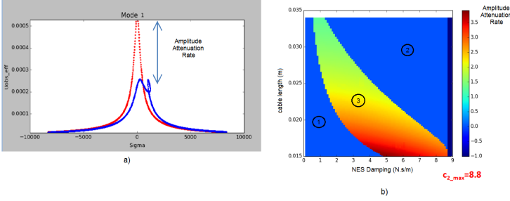
FIGURE 1: a) Fixed point response : dot line (...) denotes system response without NES and solid line (—) system response with NES b) zone 1 : The detached resonance, zone 2 : NES is not activated and zone 3 : NES is activated with Strong Modulated Response - optimal zone
