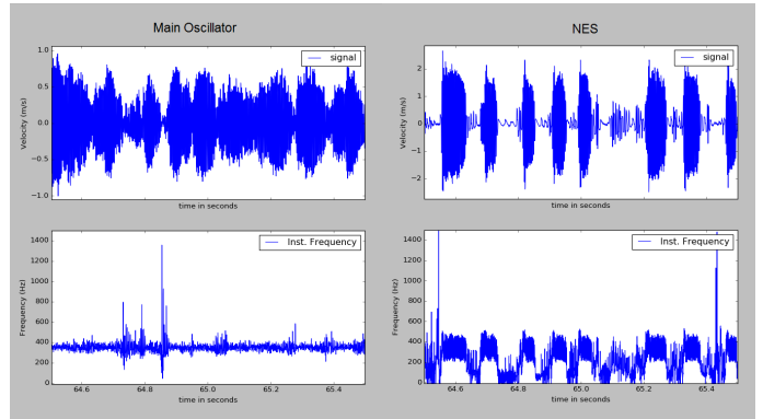
FIGURE 3: Stochastic excitation : Response on main oscillator (left) and NES (right)- Transient response (Top view) and Instantaneous Frequency (Bottom view)
