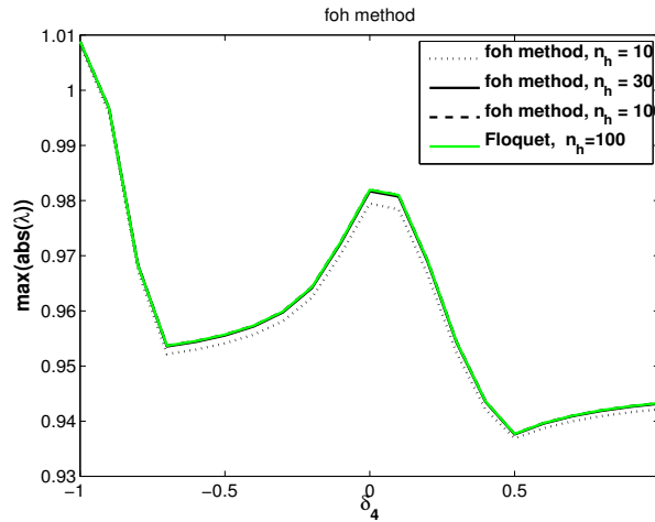
Figure 4: Evolution of the highest magnitude of the characteristic multiplier with respect to \delta_4 :
