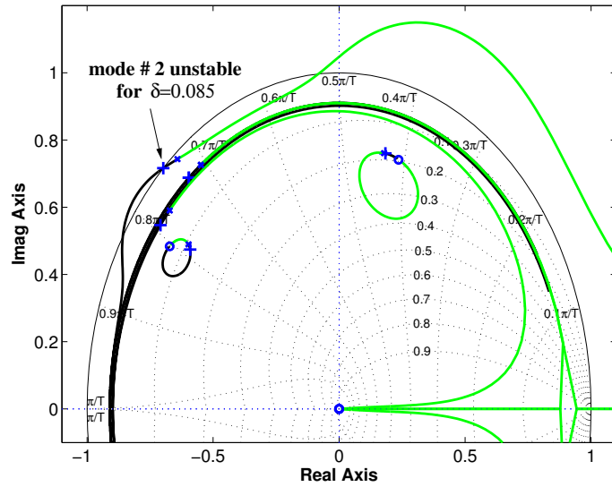
Figure 8: Characteristic multiplier loci in the z -plane according to an identical uncertainty \delta > 0 (black) or \delta < 0 (grey) on the 4 blade hinge stiffnesses at \Omega = 5 \text{ Hz} .
