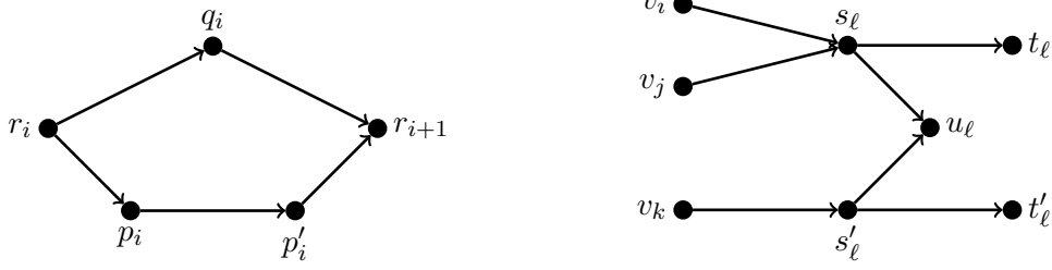
Figure 7: The two gadgets used in the proof of Theorem 24: the \{r_i, r_{i+1}\} -connector gadget (left), and the clause gadget for a clause C_\ell = x_i \vee x_j \vee x_k (right).
