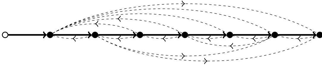
Figure 4: A planar spanned digraph (D, T) with BMRN(D, T) = 7 .
