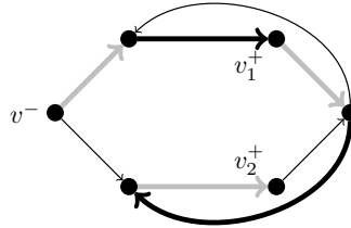
Figure 8: The out-gadget O_v . A directed Hamiltonian path P of O_v is displayed with bold arcs. The black and gray bold arcs form a 2-BPRN-colouring of (O_v, P) .
