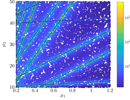
Fig. 2: Norm of the solution \|u(\mu)\|_\Sigma over the online set \mathcal{S} \subset \mathcal{P} with \#\mathcal{S} = 10^4 and \Sigma = R_X . The lines represent the resonances of the Helmholtz equation (computed analytically).
