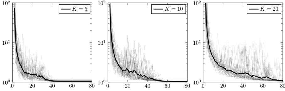
Fig. 6: Evolution of the 97.5%-quantile of \{\max\{\frac{\Delta_{\text{ref}}(\mu)}{\hat{\Delta}(\mu)}; \frac{\tilde{\Delta}(\mu)}{\Delta_{\text{ref}}(\mu)}\} : \mu \in \mathcal{P}^{\text{train}}\} during the first 80 iterations of Algorithm 3.1 . Here, n_{\tilde{\mathcal{X}}} = 30 . Each grey line corresponds to one realization of Z_1, \dots, Z_K and the black lines are the mean of the grey lines.
