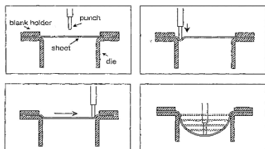
Fig. 1. Different steps of the Single Point Incremental Forming
