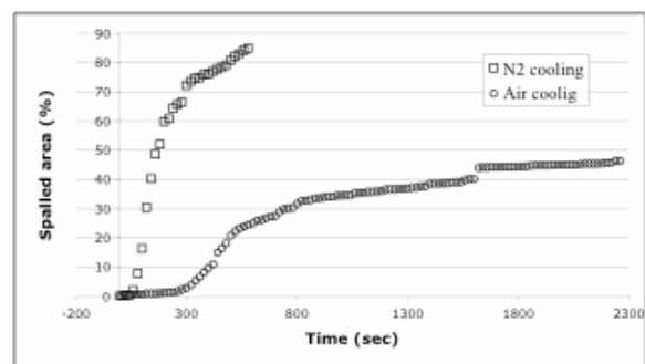
Fig. 9. Spallation kinetics of a FeCrAl alloy oxidised 384 hours at 1300°C.
