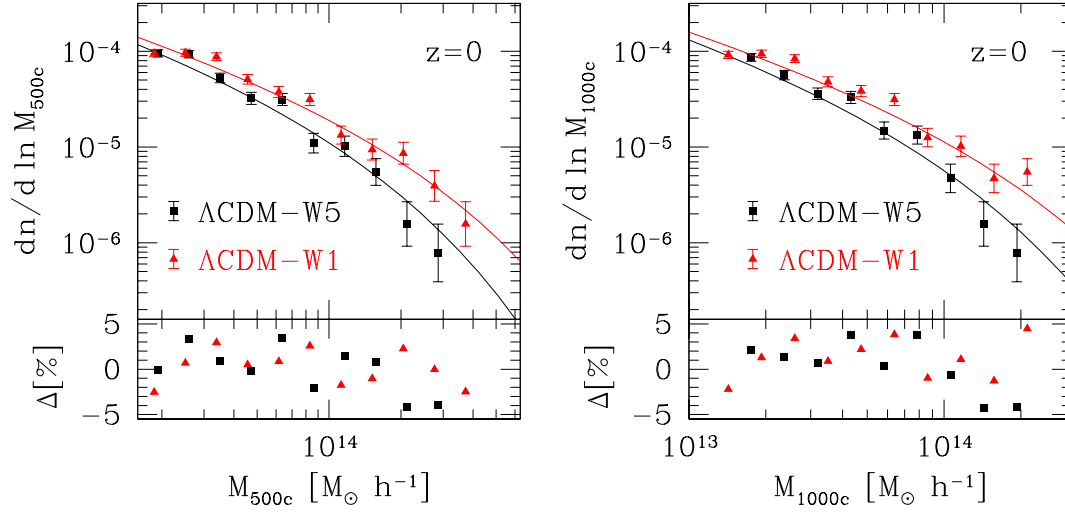
Figure 15. SOD halo mass functions from the \Lambda CDM-W5 (black squares) and \Lambda CDM-W1 (red triangles) with mass M_{500c} (left panel) and M_{1000c} (right panel) respectively against the ST-RayGal predictions.
