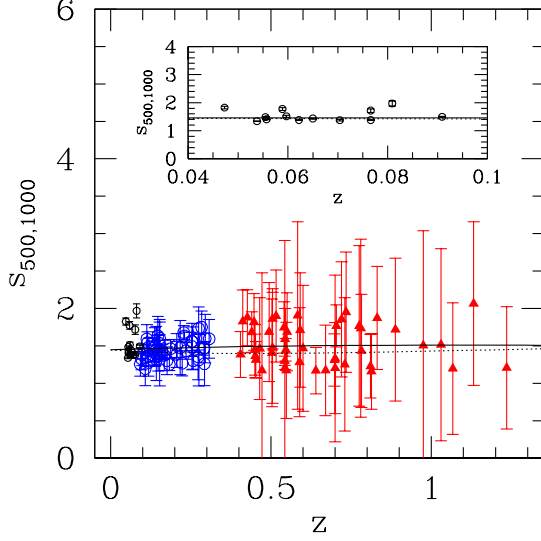
Figure 9. Sparsity of X-ray clusters. The low-redshift sample consists of clusters with mass measurements from Ettore et al. (2017a,b) and Ghirardini et al. (2017) also shown in the inset plot (black empty circles), and Ettore et al. (2010) (blue empty circles). The high-redshift sample consists of clusters with mass estimates from Amodeo et al. (2016) (red solid triangles). The black solid line and the black dotted line correspond to the best-fit \Lambda CDM models inferred assuming the ST-RayGal and ST-Despali mass functions respectively. We may notice four clusters at z < 0.1 whose sparsity significantly depart from the best-fit. We have checked that excluding these outliers from the analysis does not alter the result of the cosmological parameter inference.
