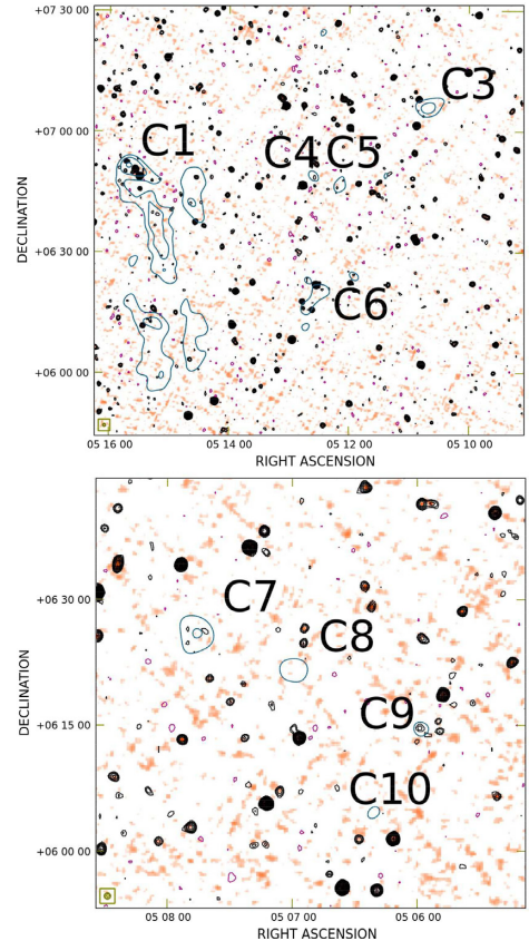
Figure 10. Region C. Left-hand panel: SRT contours ( -60, 60, 150, 500 \text{ mJy beam}^{-1} , negative in magenta and positive in black; resolution 13.9 \text{ arcmin} \times 12.4 \text{ arcmin} ) and SRT+NVSS after compact-source subtraction contours (in blue, starting from 3\sigma and the remaining increasing by a factor \sqrt{2} ; \sigma = 2.5 \text{ mJy beam}^{-1} , resolution 3.5 \text{ arcmin} \times 3.5 \text{ arcmin} ) overlaid on X-ray emission from the RASS in red colours and radio emission from the SRT+NVSS (resolution 3.5 \text{ arcmin} ) in grey colours. Right-hand panels: NVSS contours -3\sigma (magenta, \sigma = 0.45 \text{ mJy beam}^{-1} ), 3\sigma , and increasing by a factor \sqrt{2} (black) overlaid on the TGSS in colours. The black arrow marks the position of A539. The colorbars are the same as in Fig. 7.
