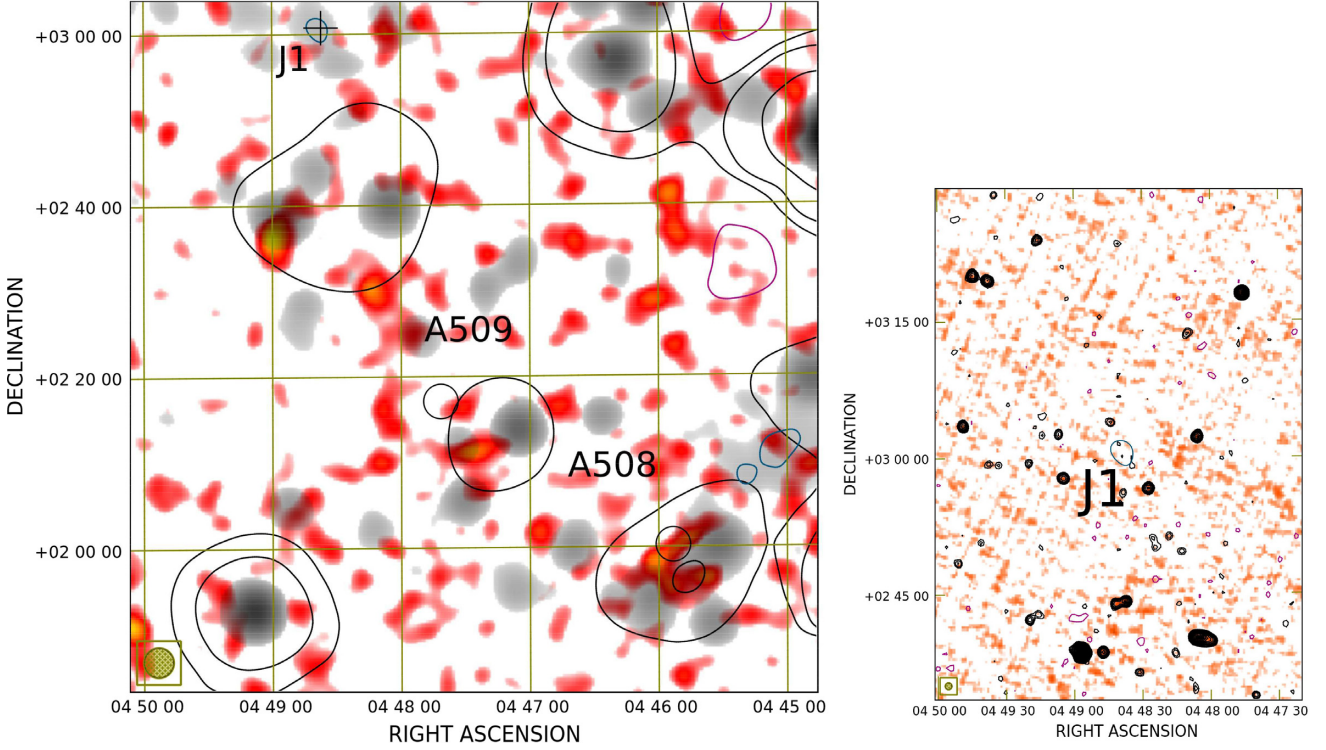
Figure 17. Region J. Left-hand panel: SRT contours ( -60, 60, 150, 500 mJy beam ^{-1} , negative in magenta and positive in black; resolution 13.9 arcmin \times 12.4 arcmin) and SRT+NVSS after compact-source subtraction contours (in blue, starting from 3\sigma and the remaining increasing by a factor \sqrt{2} ; \sigma = 2.5 mJy beam ^{-1} , resolution 3.5 arcmin \times 3.5 arcmin) overlaid on X-ray emission from the RASS in red colours and radio emission from the SRT+NVSS (resolution 3.5 arcmin) in grey colours. Right-hand panel: NVSS contours -3\sigma (magenta, \sigma = 0.45 mJy beam ^{-1} ), 3\sigma , and increasing by a factor \sqrt{2} (black) overlaid on the TGSS in colours. The colorbars are the same as in Fig. 7.
