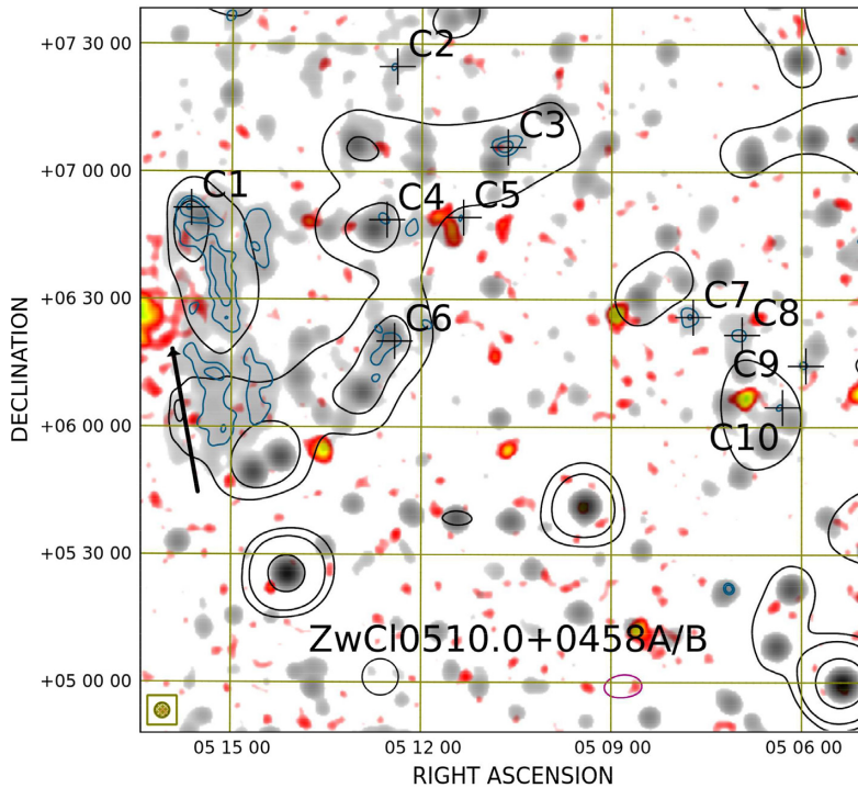
Figure 10. Region C. Left-hand panel: SRT contours ( -60, 60, 150, 500 \text{ mJy beam}^{-1} , negative in magenta and positive in black; resolution 13.9 \text{ arcmin} \times 12.4 \text{ arcmin} ) and SRT+NVSS after compact-source subtraction contours (in blue, starting from 3\sigma and the remaining increasing by a factor \sqrt{2} ; \sigma = 2.5 \text{ mJy beam}^{-1} , resolution 3.5 \text{ arcmin} \times 3.5 \text{ arcmin} ) overlaid on X-ray emission from the RASS in red colours and radio emission from the SRT+NVSS (resolution 3.5 \text{ arcmin} ) in grey colours. Right-hand panels: NVSS contours -3\sigma (magenta, \sigma = 0.45 \text{ mJy beam}^{-1} ), 3\sigma , and increasing by a factor \sqrt{2} (black) overlaid on the TGSS in colours. The black arrow marks the position of A539. The colorbars are the same as in Fig. 7.
