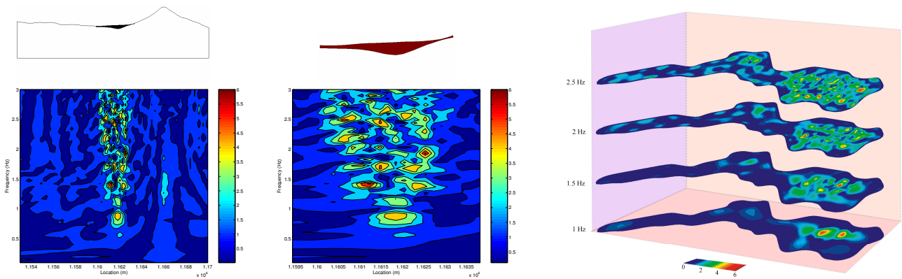
Figure 4. Spectral ratio for the NS velocity component due to a NS polarized plane S wave, along the LPG profile including the topography (left), along the LPG profile restricted to the basin section (middle) and for the entire basin for frequencies from 1 to 2.5Hz (right).
