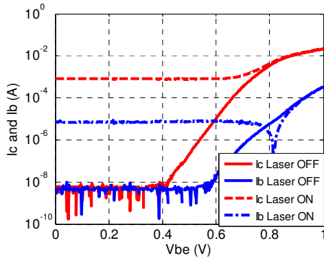
Figure 2: Gummel plot under 2.28 mW optical power illumination and dark conditions.
