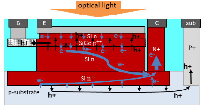
Figure 3: the schematic that indicates the flow of photo-generated carriers that are generated at different region of the HPT.
