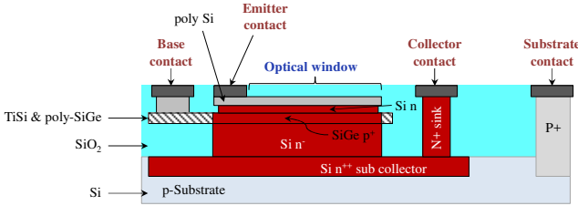
Figure 1: Simplified schematic cross-section of HPT with extended Emitter, Base and Collector regions.
