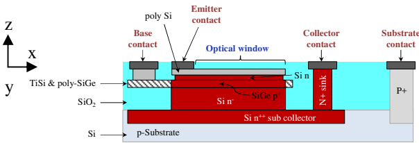
Figure 2: Simplified schematic cross-section of an extended Emitter Base Collector HPT
