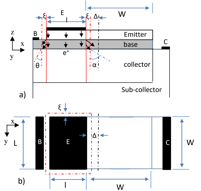
Figure 9: The simplified a) cross-sectional and b) top view of the transistor that indicates the impact of the peripheral region \xi , the collector current spreading region \theta and lateral extension into the optical window \Delta .
