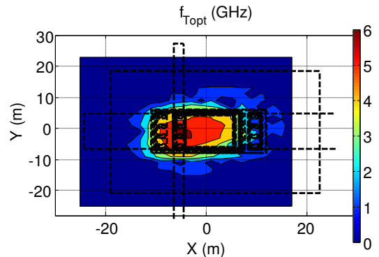
Figure 15: The topological map of the optical transition frequency f_{T_{opt}} at various locations of optical light illumination.
