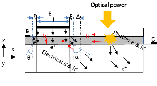
Figure 12: The simplified cross-sectional view of the phototransistor that indicates the peripheral region \xi and its dissymmetric enlargement \Delta , the collector current spreading region \theta , and the photo-generated carrier flow.
