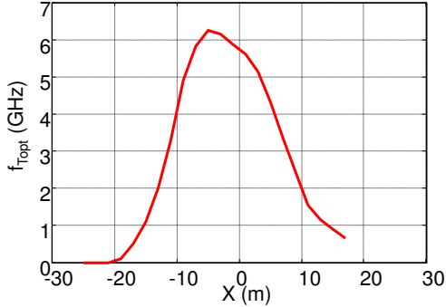
Figure 16: The slice curve of the optical transition frequency f_{\text{Topr}} at Y=0 \mu\text{m}
