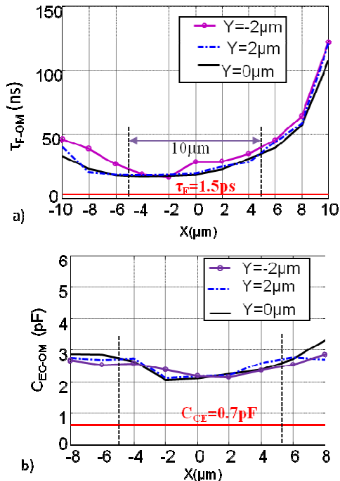
Figure 17: The extracted opto-microwave a) forward transit time and b) emitter-collector junction capacitance at different optical injection positions over the phototransistor optical window. The electrical forward transit time ( \tau_{\text{F}} ) and emitter-collector capacitance ( C_{\text{EC}} ) are plotted in figures a) and b) respectively.
