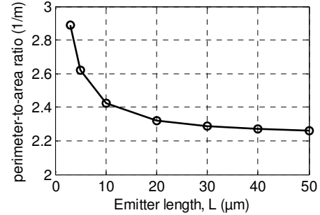
Figure 5: The perimeter to area ratio of various size HBTs versus emitter length with a constant emitter width l = 0.9\ \mu\text{m}
