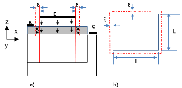
Figure 3: Schematic a) cross-section and b) top view of the HBT of length L and width l to illustrate the influence of the peripheral region over the extension \xi .
