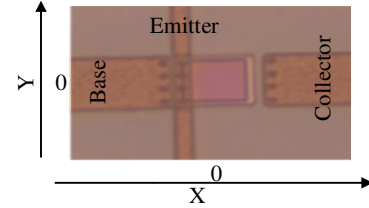
Figure 14: The microscopic picture of the top view of the transistor.
