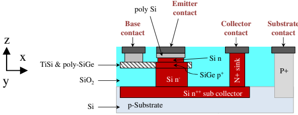
Figure 1: Schematic cross-section of SiGe2RF technology from Telefunken
