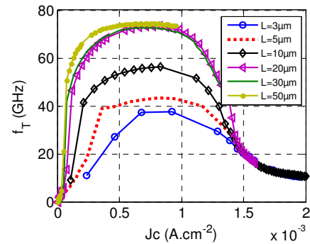
Figure 6: f_T versus collector current density for different emitter length HBTs with a constant emitter width of 0.9\ \mu\text{m}
