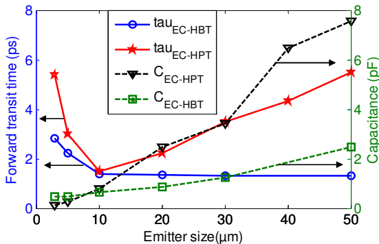
Figure 10: The extracted electrical transit time and junction capacitances as a function of emitter length L for HBT (with l=0.9 \mu\text{m} ) and HPT (with l=L ) structures.
