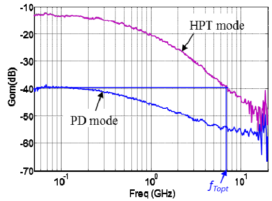
Figure 11: Opto-microwave gain in the photodiode ( V_{be}=0 \text{ V} , V_{ce}=3 \text{ V} ) and phototransistor ( V_{be}=0.857 \text{ V} , V_{ce}=3 \text{ V} ) modes of 10 \times 10 \mu\text{m}^2 optical window HPT.
