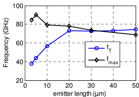
Figure 4: f_T and f_{max} of HBTs as a function of emitter length L with a constant emitter width l = 0.9\ \mu\text{m} and for V_{ce} = 3.5\ \text{V} .
