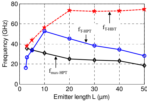
Figure 8: f_{T-HPT} , f_{T-HBT} and f_{max-HPT} as a function of emitter length L for a constant emitter width of l=0.9 \mu\text{m} . For HPTs, the optical window W and emitter length L as shown in Figure 9 have equal dimension whereas for HBTs W=0 \mu\text{m} along x -axis.
