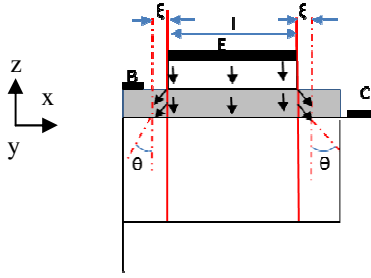
Figure 7: The simplified cross-sectional view of the transistor that indicates the impact of the peripheral current and the collector current spreading. The \theta is the angle of current spreading in the collector.
