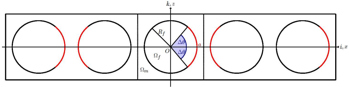
Figure 1. Schematic representation of a single “free” 90° ply with debonded fibers.
