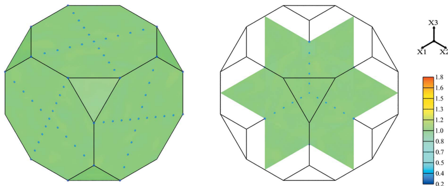
Figure 10 Generation of a uniform orientation distribution in the presence of prescribed orientations. Case of 1000 orientations among which 82 are prescribed, which are located along the X_1\parallel(100) and X_1\parallel(110) fibres. The prescribed orientations are shown by blue dots and the colour field represents the ODF. Cubic crystal symmetry is considered. ODFs are shown as surface and slice views. Note that the ODF is as uniform as in the standard case (Fig. 5a).
