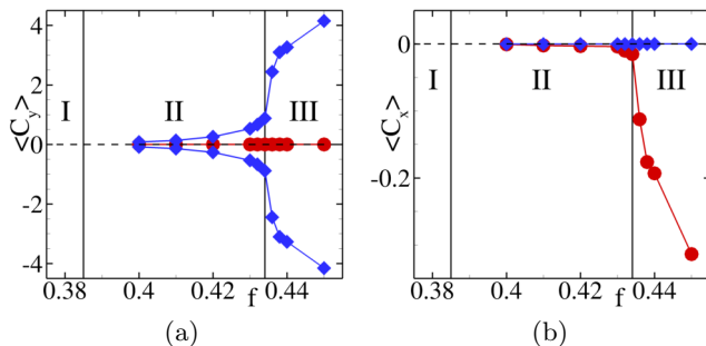
FIG. 18. Mean lift and drag coefficients for the symmetric \mathbf{u}_s'' (red circles) and anti-symmetric \mathbf{u}_a'' (blue diamonds) components as a function of the flapping frequency f .
